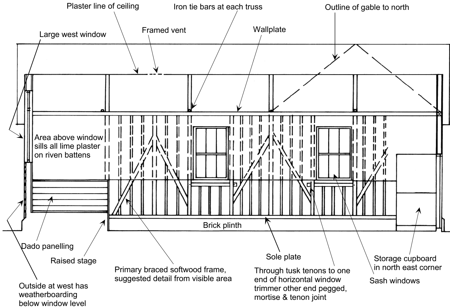
LONG SECTION LOOKING NORTH
