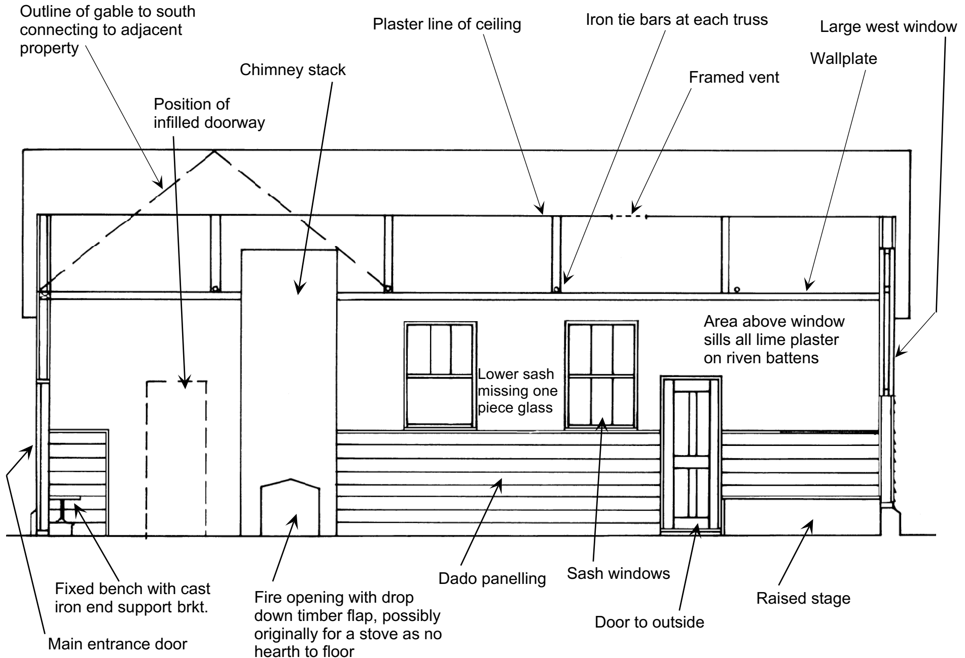
LONG SECTION LOOKING SOUTH
