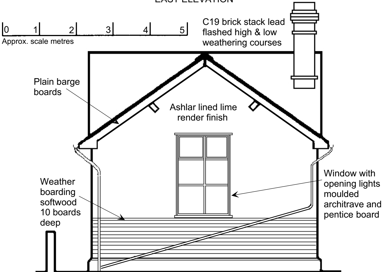
WEST ELEVATION
