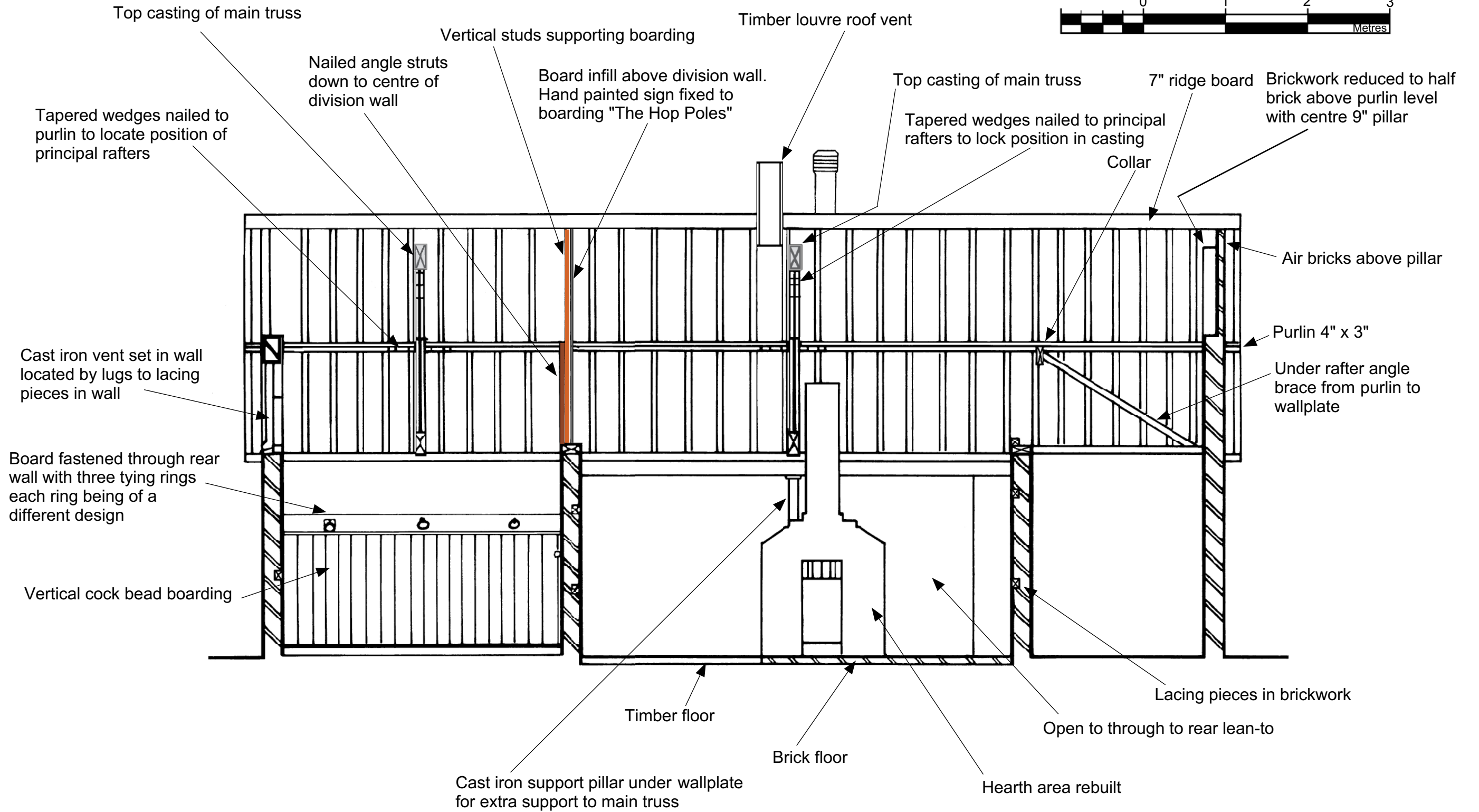
LONG SECTION LOOKING NORTH
