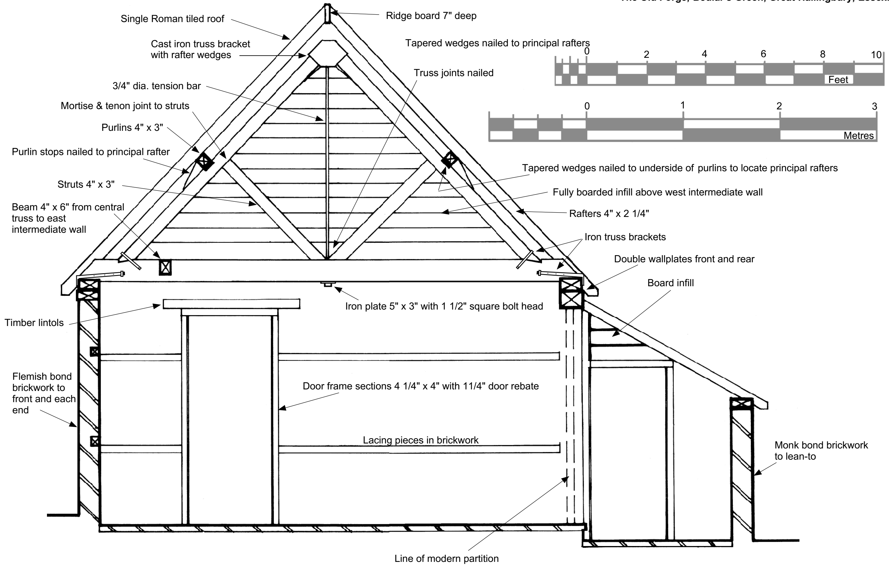
SECTION THROUGH BUILDING LOOKING WEST
