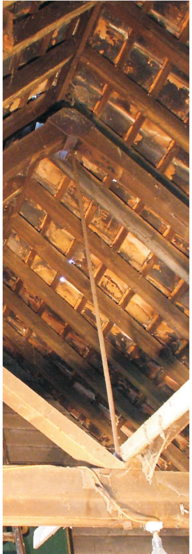
Centre of truss with tension bar and base of purlin struts. Small iron hook, use unknown near centre of tiebeam
