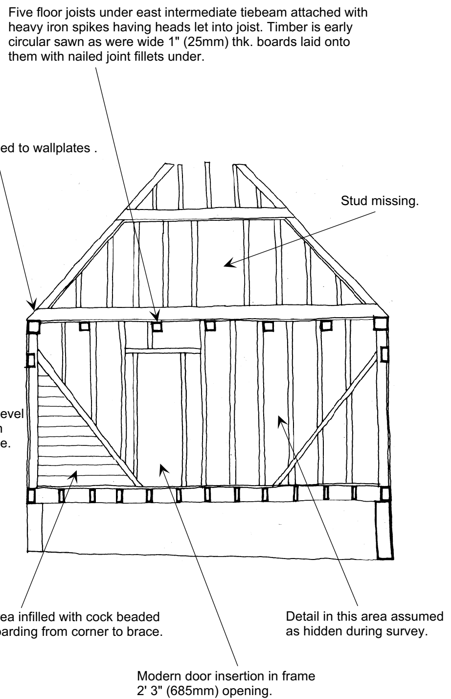
SECTION "D" - "D" East end wallframe from inside.
