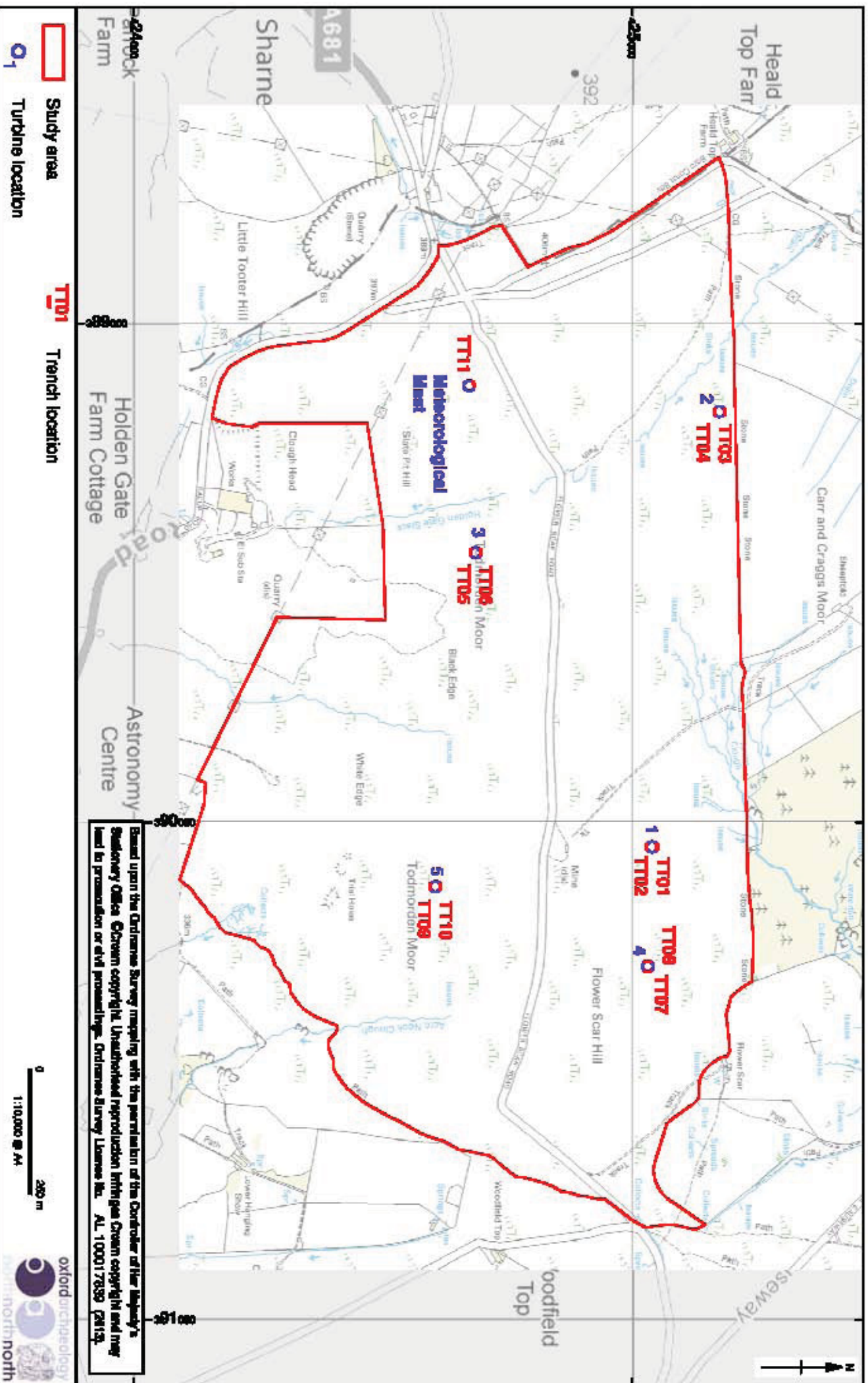
Figure 2: Tidal trench locations
