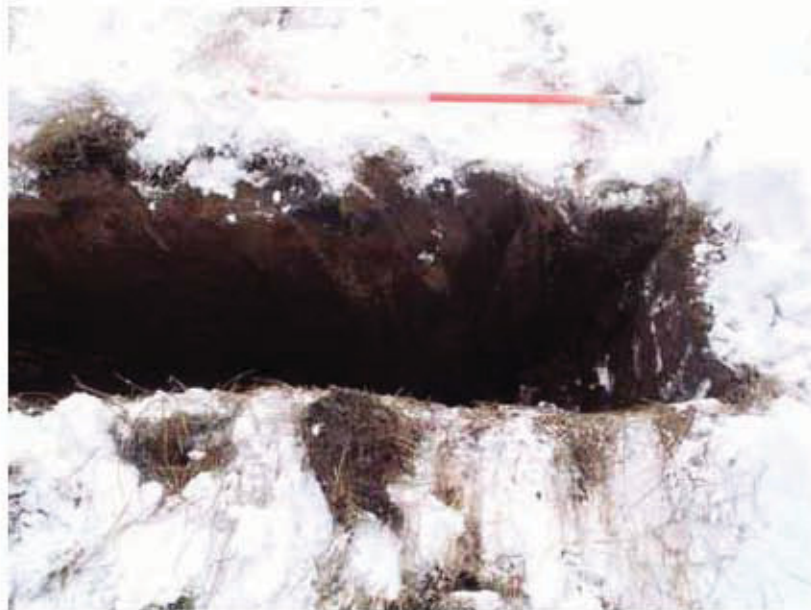
Plate 2: North-facing section of TT04
