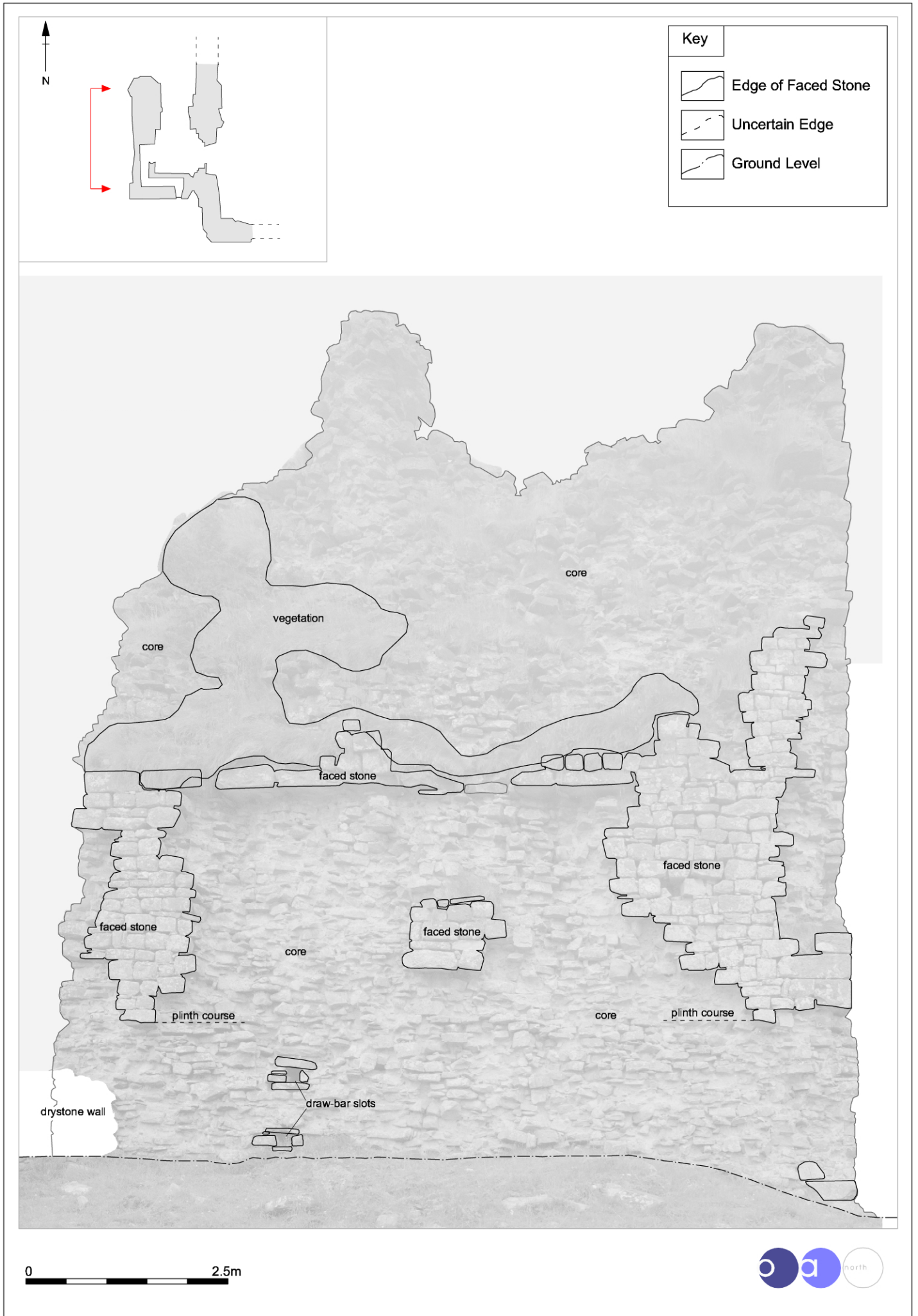
Figure 15: West external elevation of the barban
