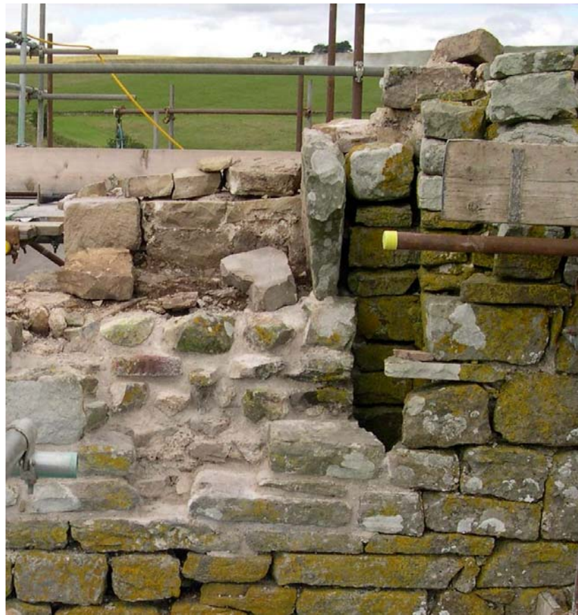
Plate 14: Garderobe revealed at parapet level, south elevation of the barbican
