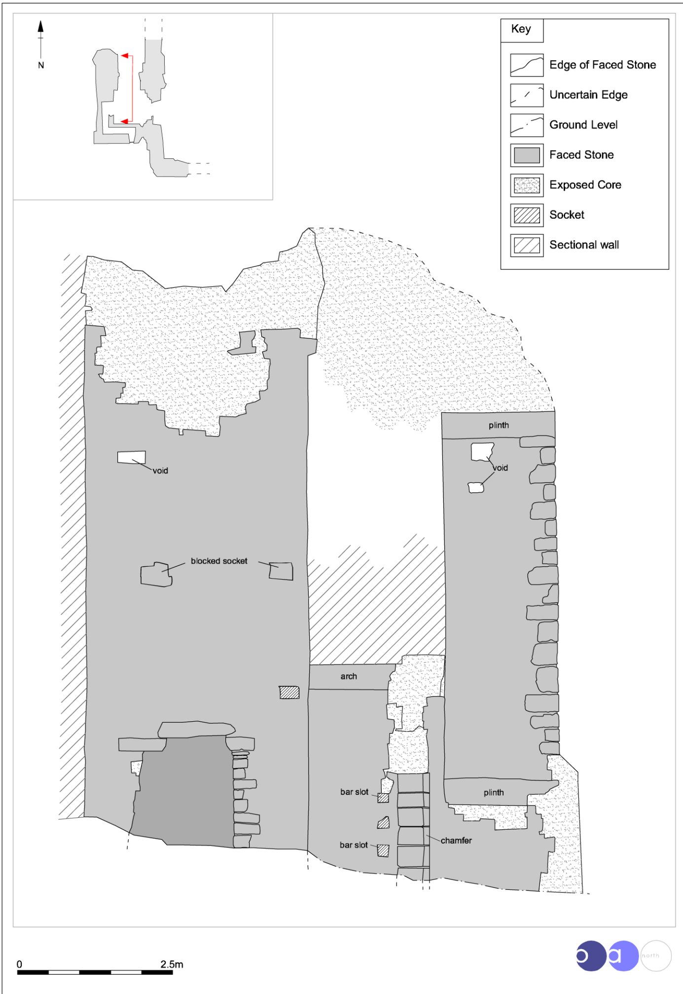
Figure 14: West internal elevation of the barbican
