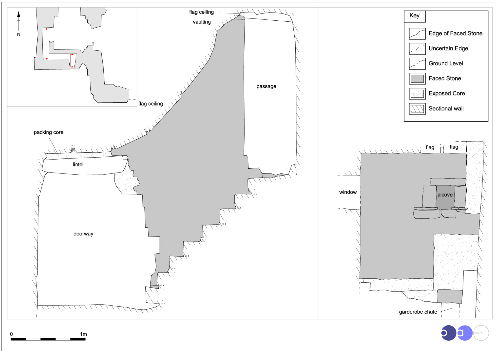
Figure 17: West-facing internal elevations of the barbican garderobe
