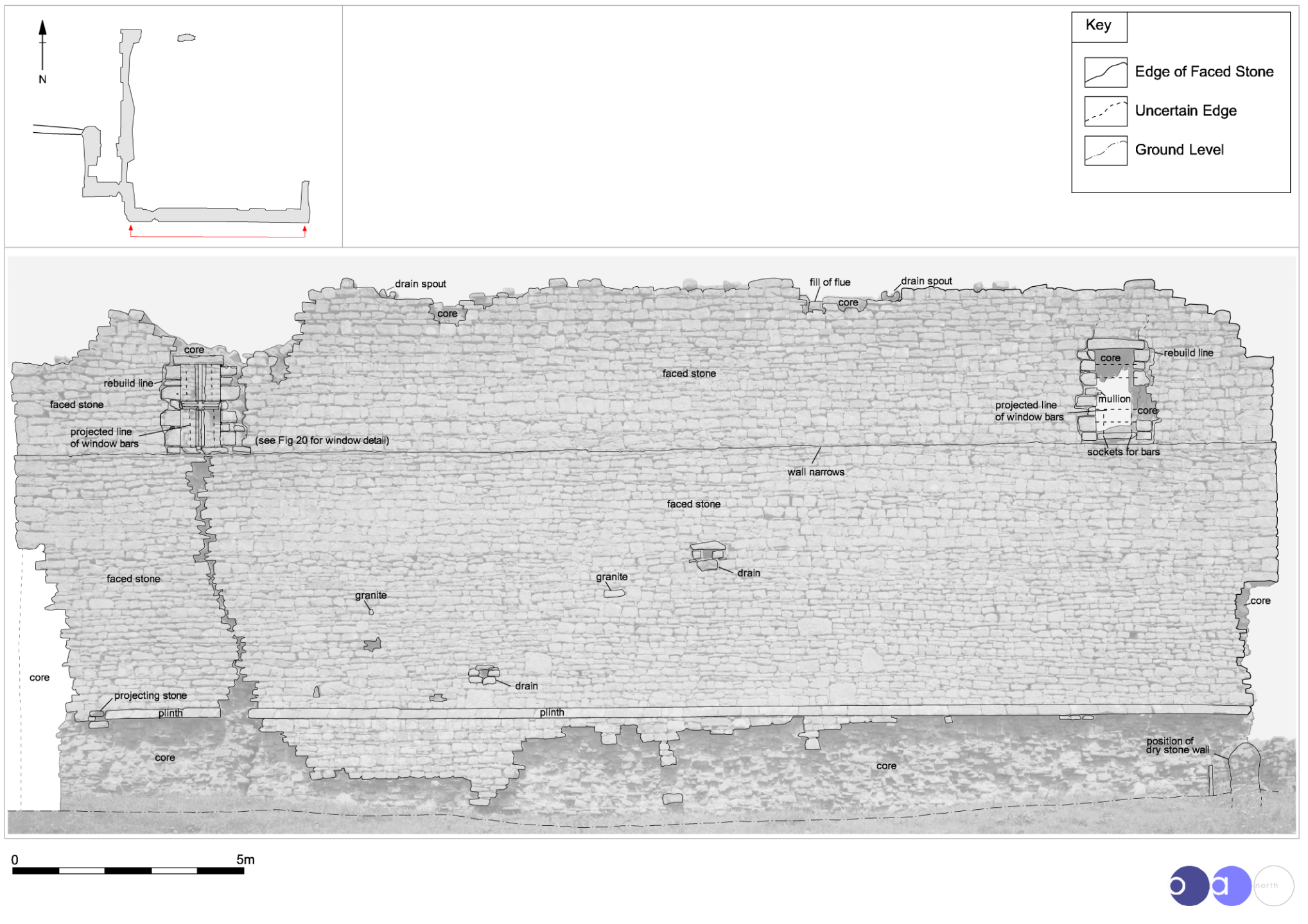
Figure 3: South external elevation of the castle
