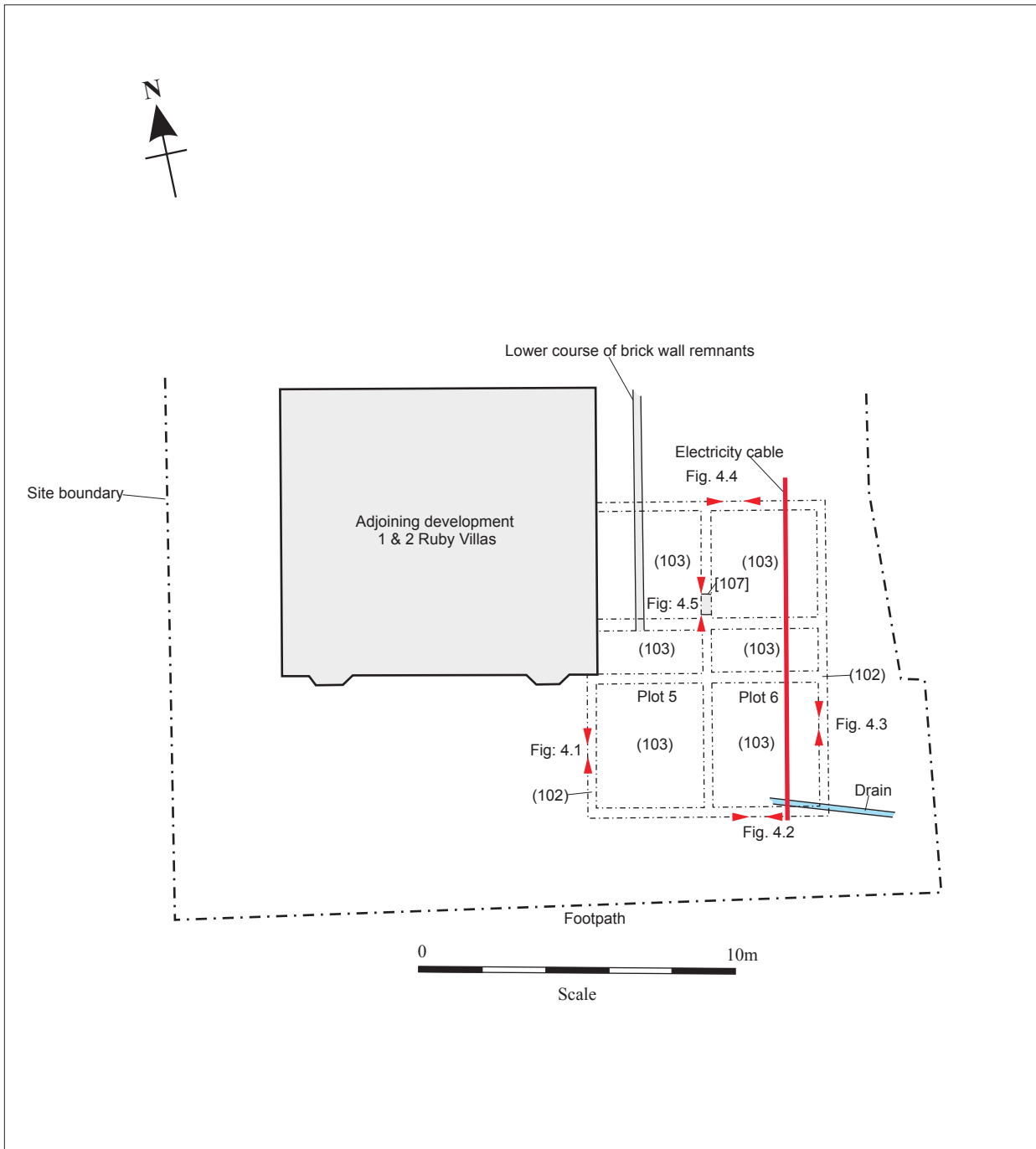
Fig. 3. Plan of Plots 5 & 6. Scale 1:200
