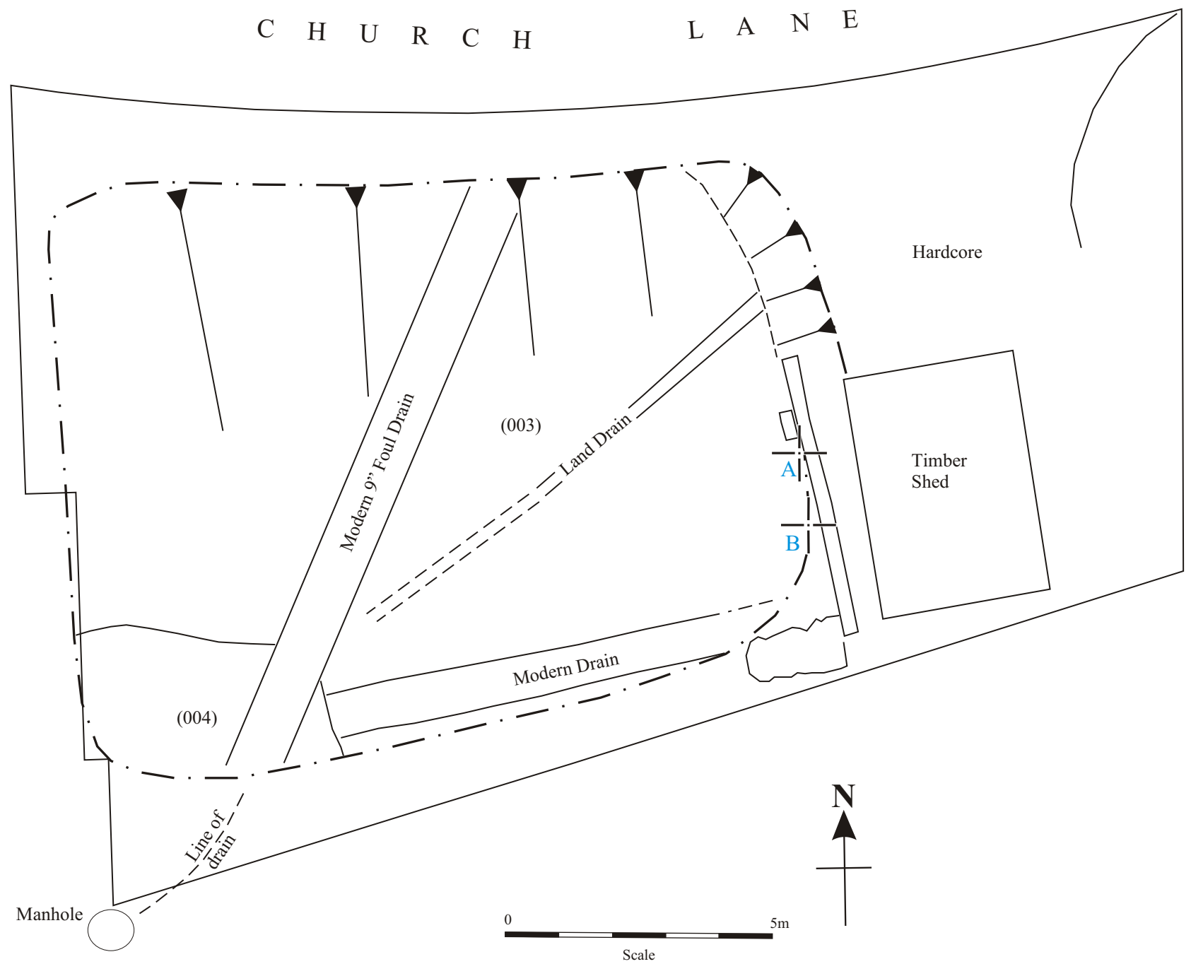
Fig. 3: Plan of the development area after the topsoil and subsoil had been stripped. Scale 1:100
