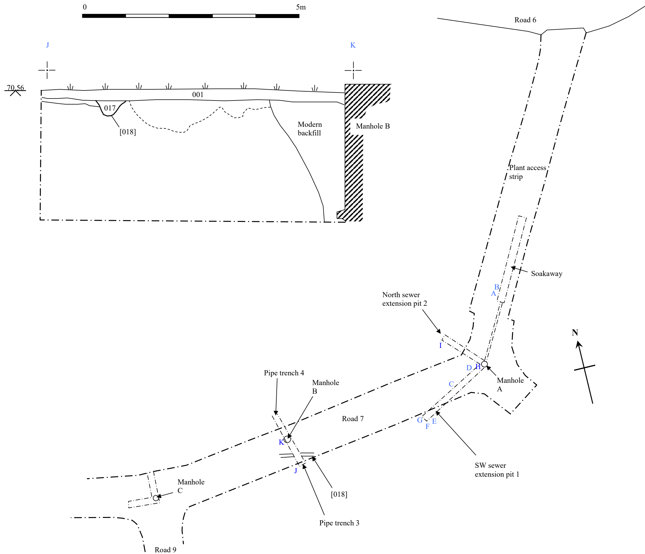
Figure 4: Plan of the Road 7 and plant access road strips with associated groundworks at scale 1:500, with section drawings at 1:20 and 1:50. Additional section drawings appear in figure 5.
