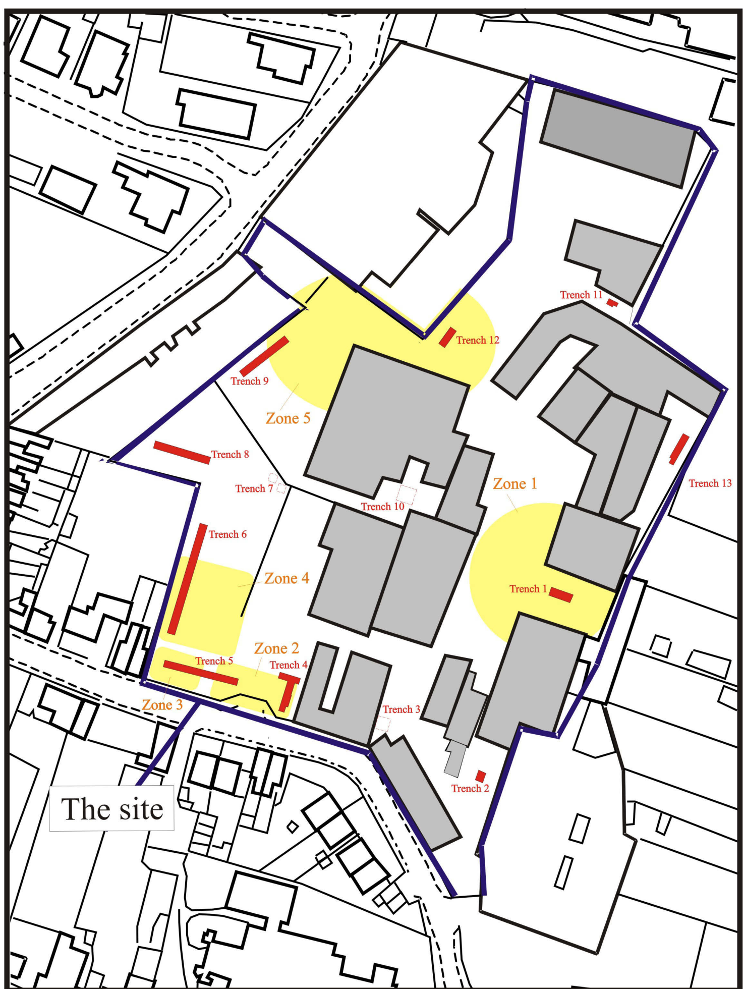
Figure 2: Site plan showing the site boundary, the trenches outlined in red, and the identified zones of archaeological potential in yellow. (Scale 1:2000)
