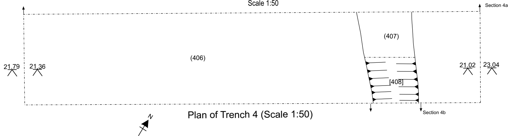
Figure 6 Plan and Sections of Trench 4 (Scale 1:50)
