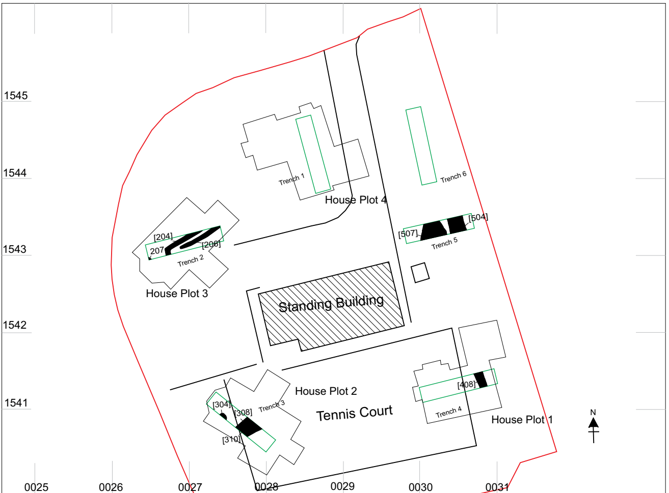
Figure 3 Trench Location Plan (Scale 1:500)
