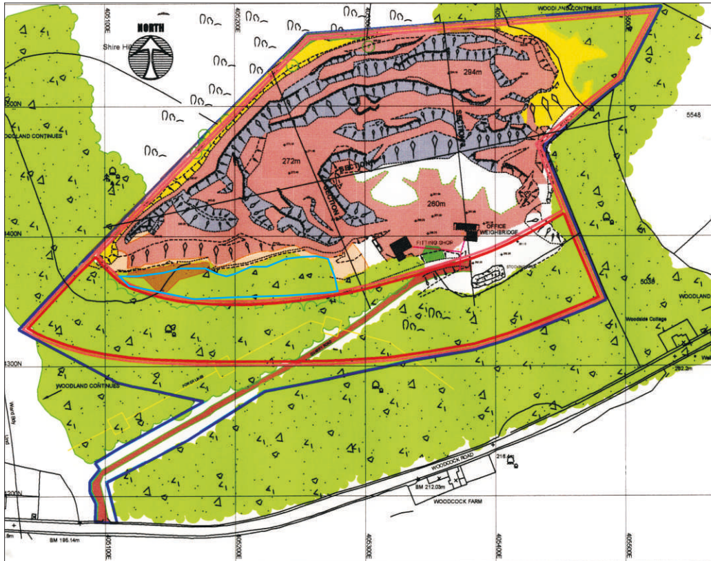
Figure 7 Proposed extent of quarry works (Scale 1:4000)
