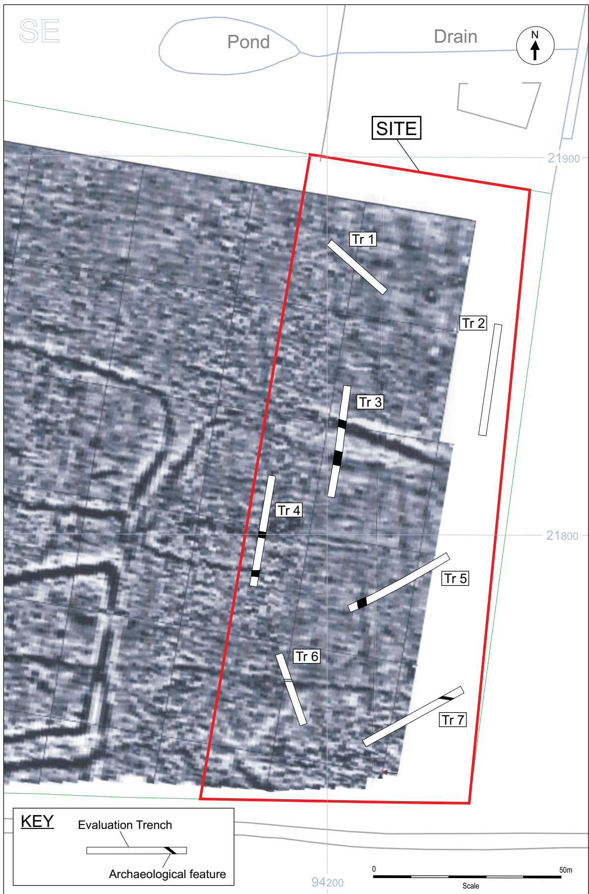
Fig. 2 Trench location plan superimposed over the results of the Geophysical Survey Scale 1:1000
