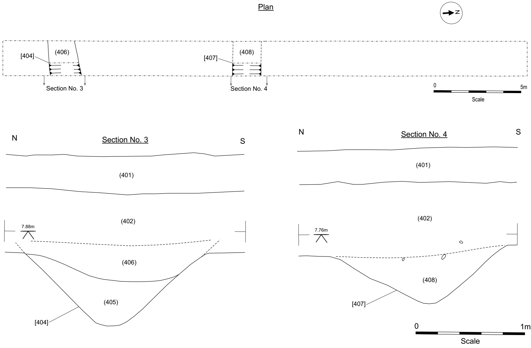
Fig. 5 Trench 4 Plan 1:120, Sections 1:20
