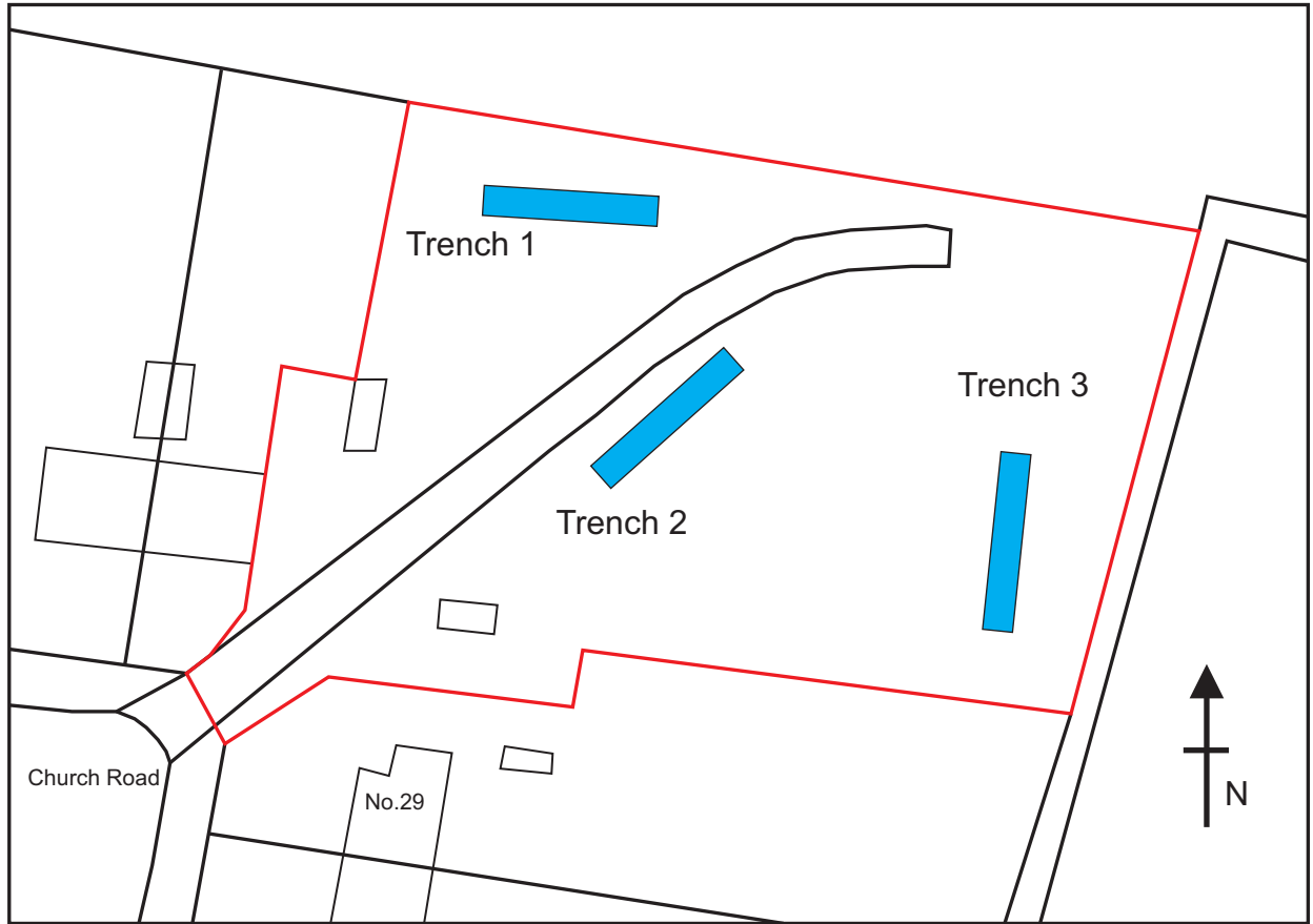
Fig. 2: Trench location plan (Scale 1:500) @A4
