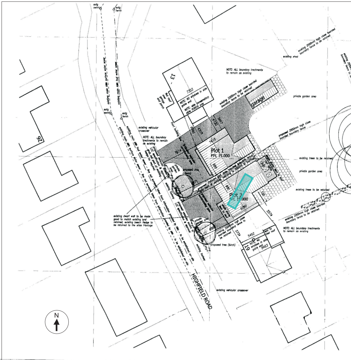
Fig. 2: Trench Layout
