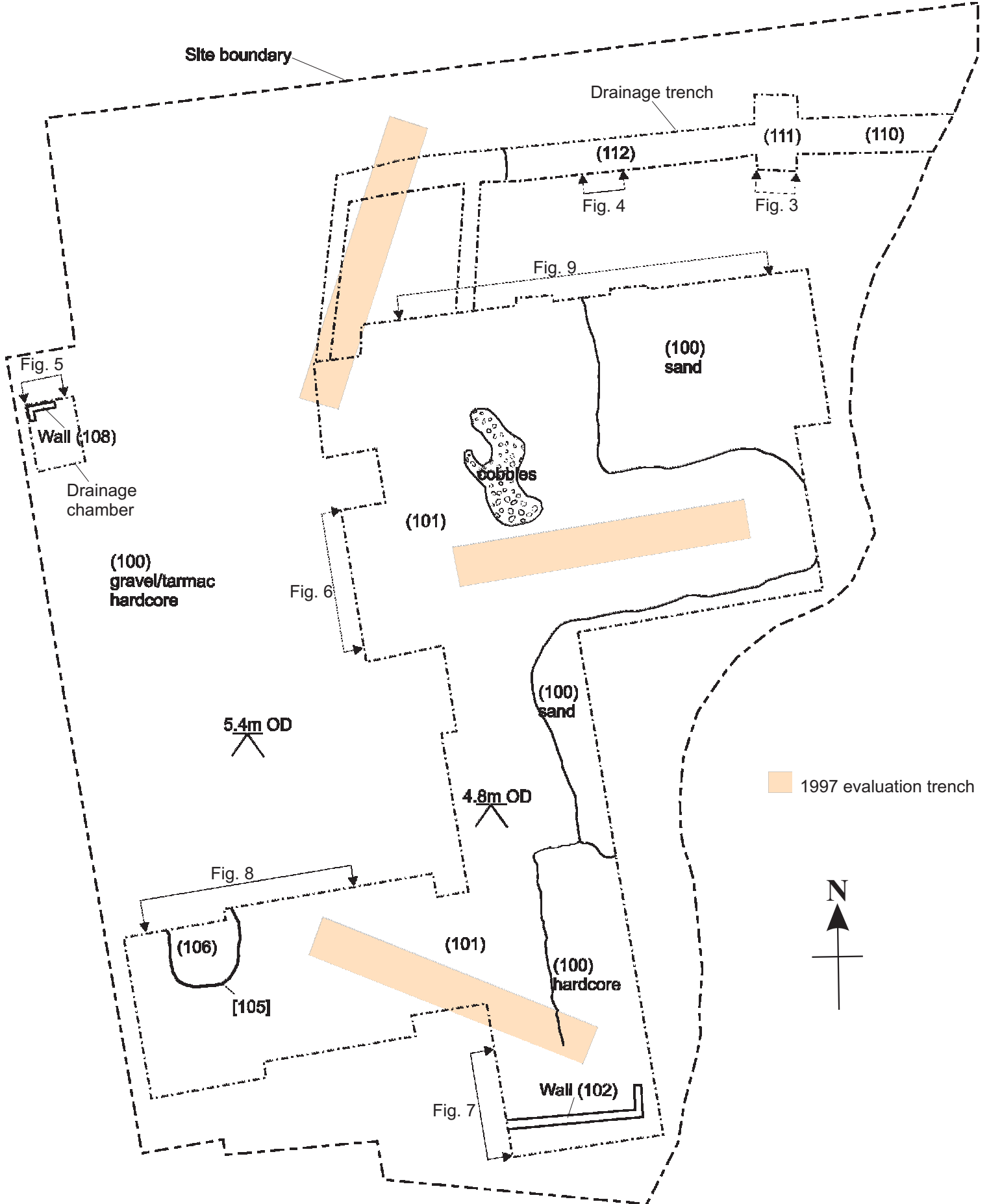
Figure 2 Site plan with 1997 evaluation trenches Scale 1:250
