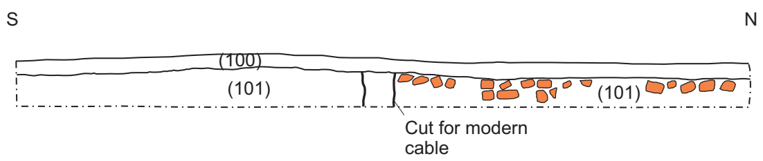
Figure 6 East facing section through layer (101) Scale 1:50
