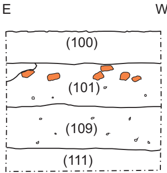
Figure 3 North facing section of drainage manhole Scale 1:50
