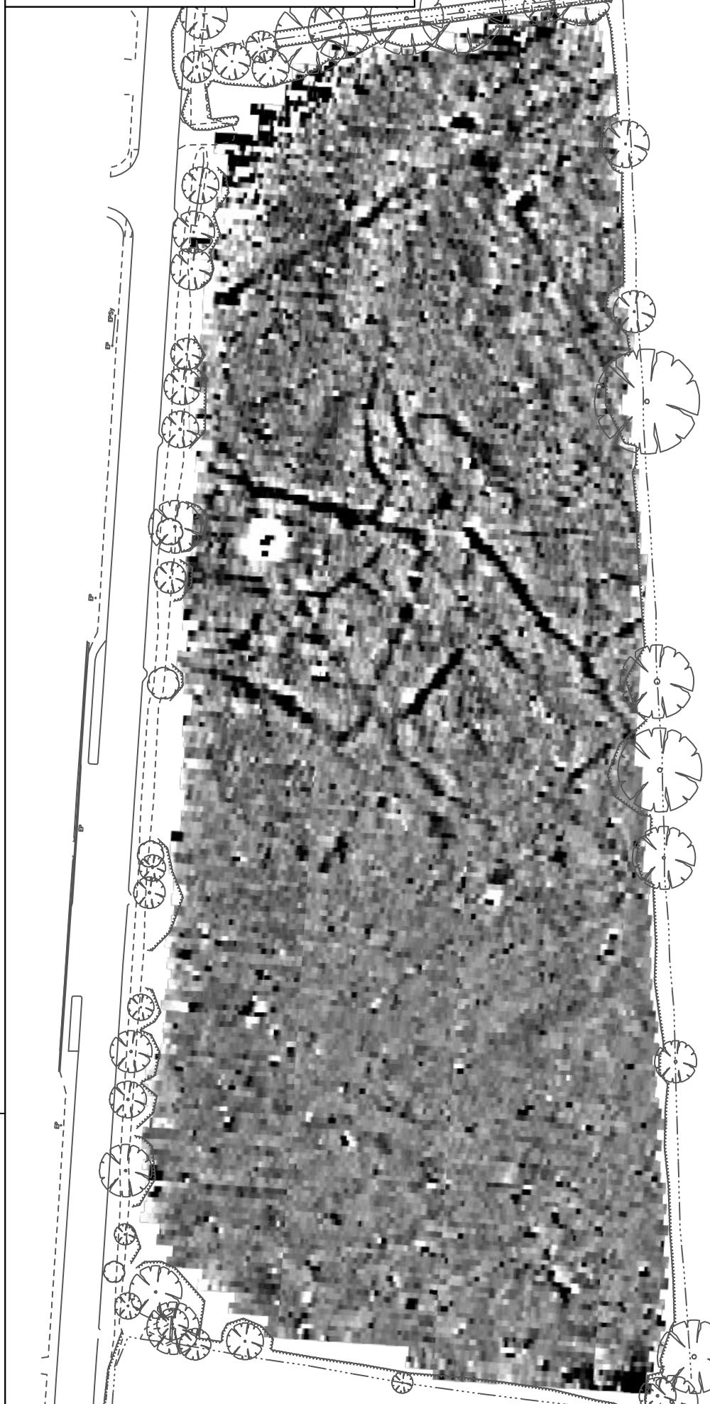
PLOT OF MINIMALLY PROCESSED GRADIOMETER DATA
