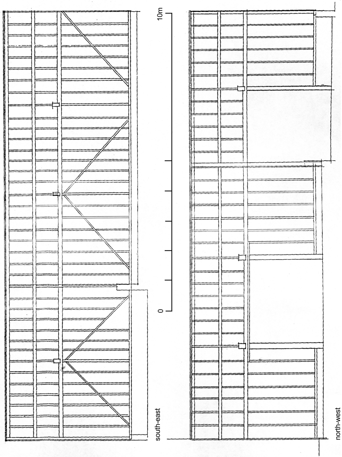
Fig 8d Building (D) attached to barn (E): internal elevations - of south-east side and north-west side, and cross-sections.
