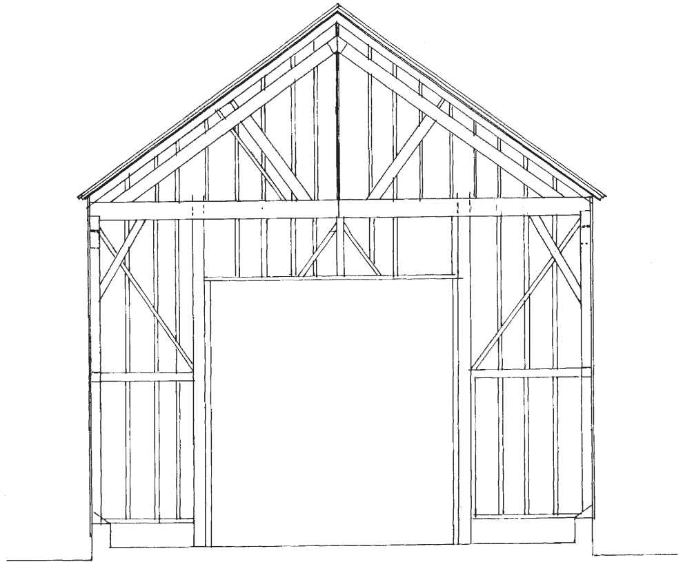
south-east gable
