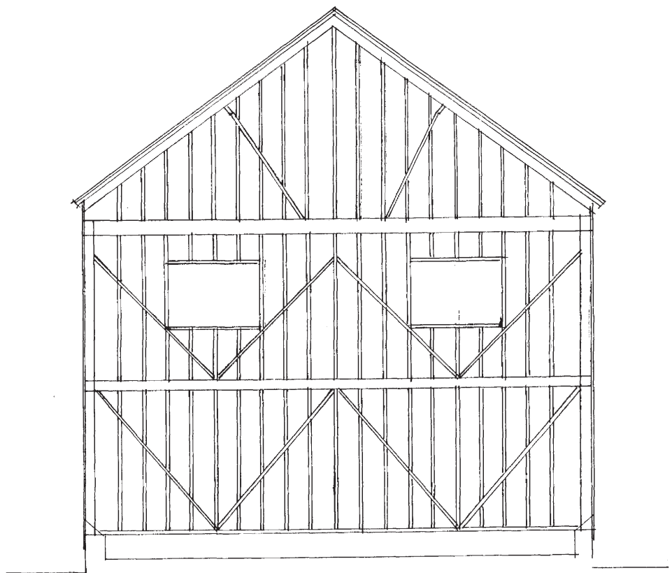
north-west gable
