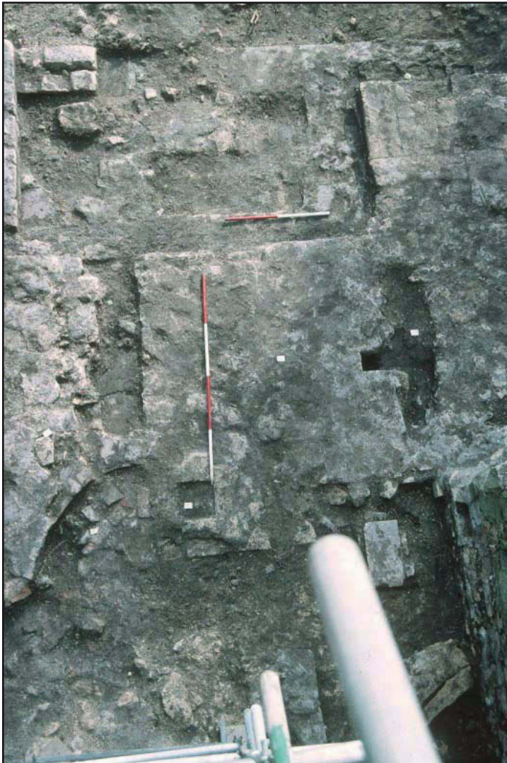
Plate 3: Building 5a seen from above and north. Suggested steam engine position at top and boiler position below
