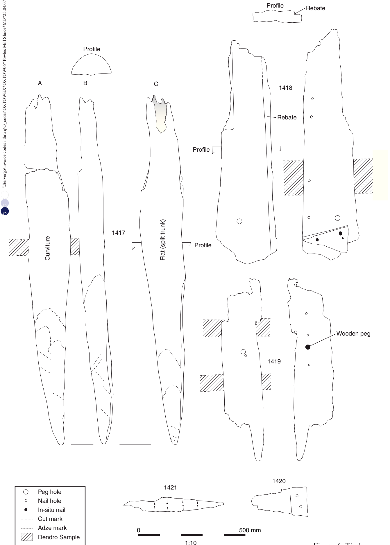
Figure 6: Timbers
