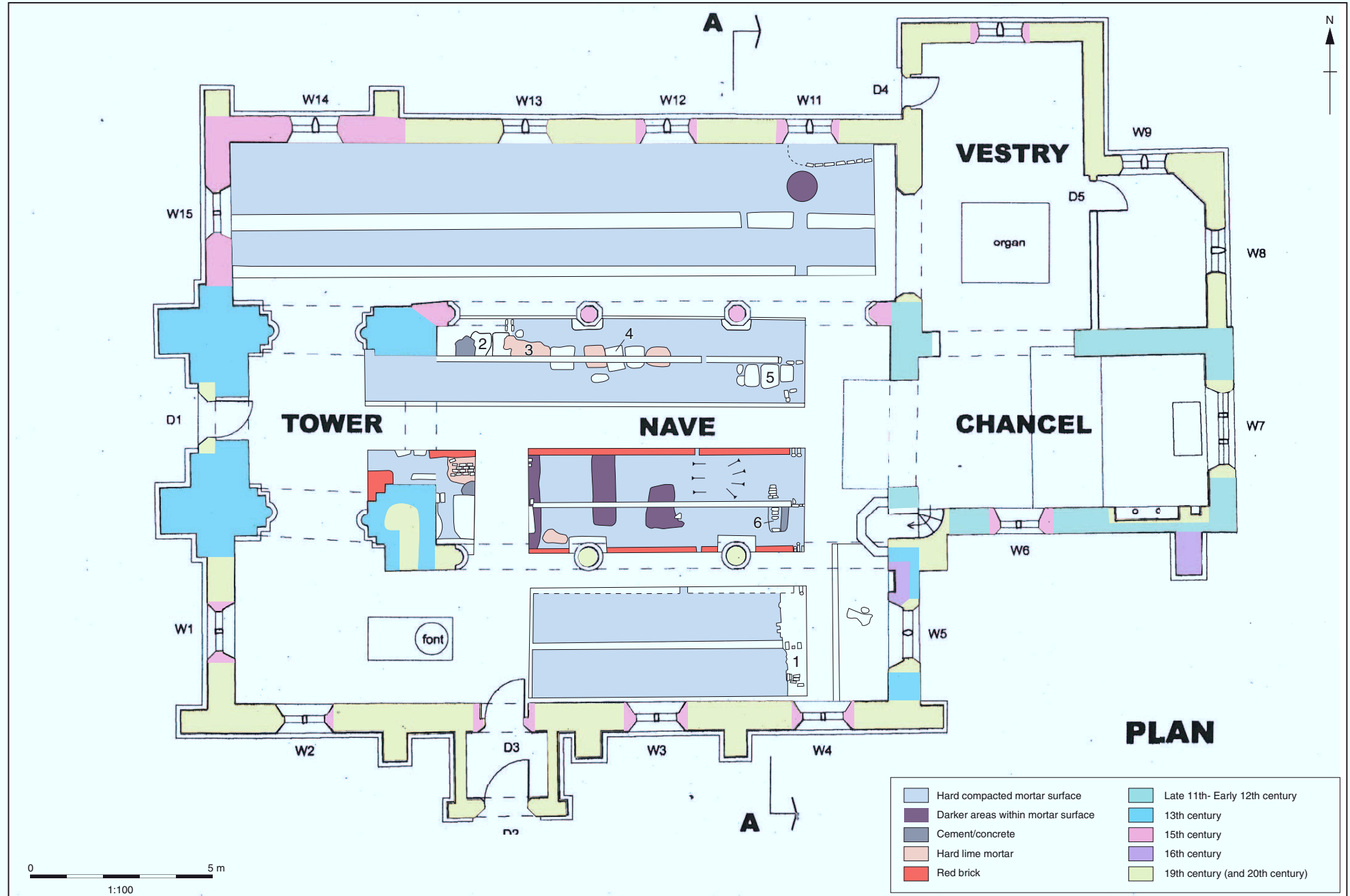
Figure 2: Phasing plan of St Cross Church
