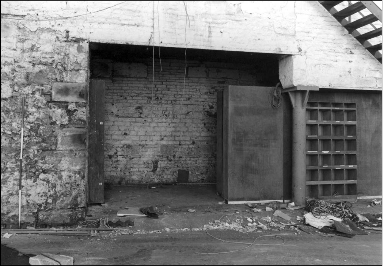
Photo 29: Building 1: interior view of south wall, showing inserted opening with column (film 3, frame 5)
