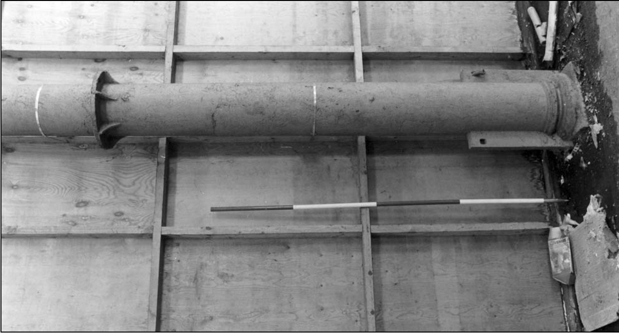
Photo 11: Building 1: detail of lower part of column, west side (film 3, frame 18)
