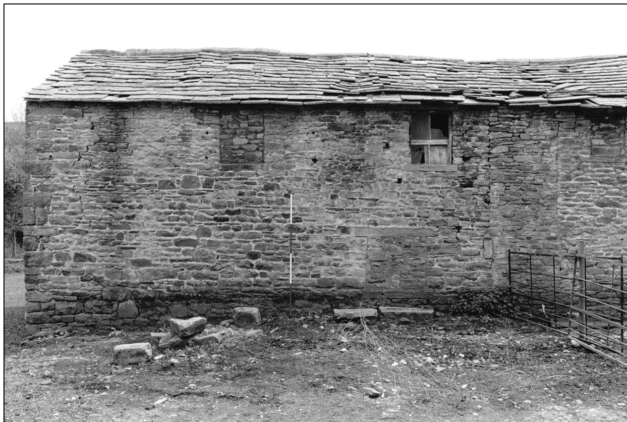
Photo 16: Power House: north-west elevation (left part)
