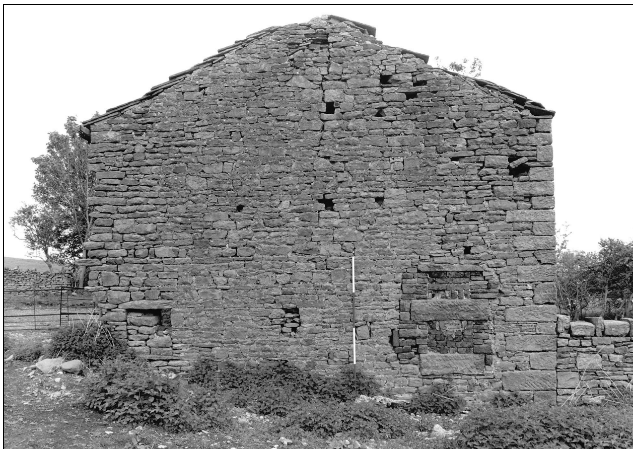
Photo 13: Power House: south-west gable
