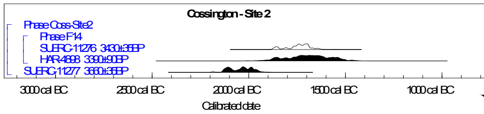
Figure 80: Probability distributions of dates from Barrow 2 (Site area 2).
