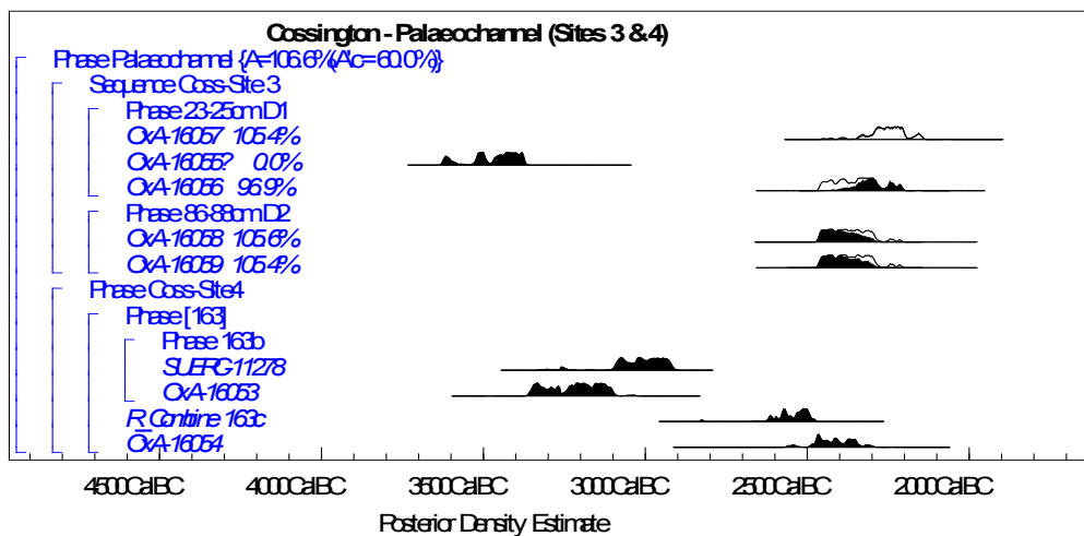
Figure 83 Probability distributions of dates from Area D palaeochannel (Site areas 3 and 4). Each distribution represents the relative probability that an event occurs at a particular time. For each of the radiocarbon dates two distributions have been plotted, one in outline, which is the result of simple radiocarbon calibration, and a solid one, which is based on the chronological model used. The large square brackets down the left hand side along with the OxCal keywords define the model exactly.
