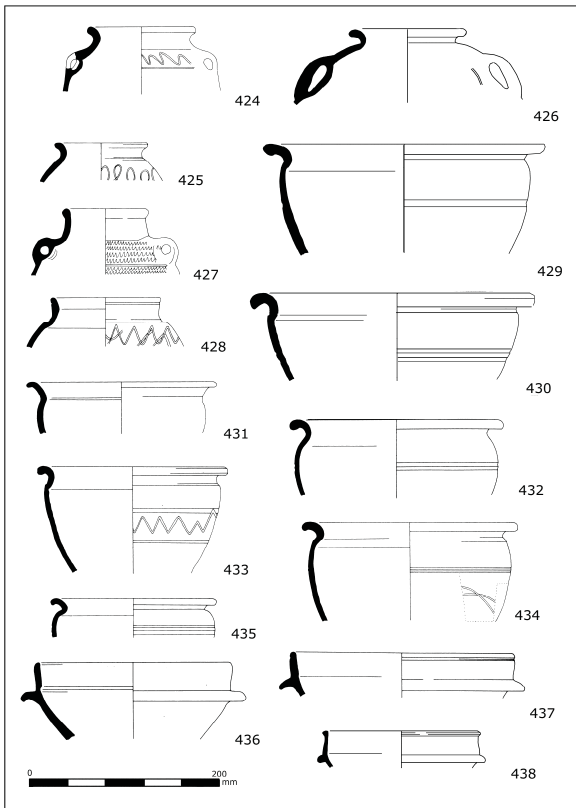
Fig. D9.57. Coarse pottery type series nos. 424-438. Scale 1:4.
