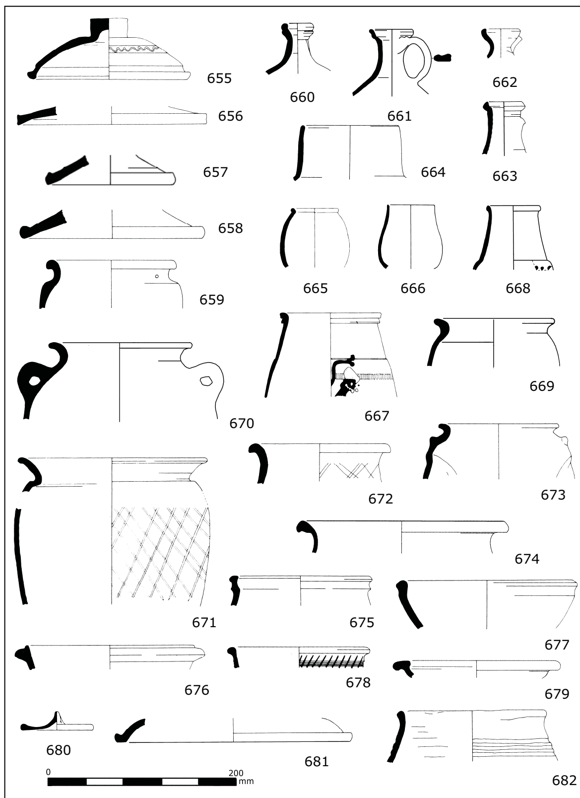
Fig. D9.67. Coarse pottery type series nos. 655-682. Scale 1:4.
