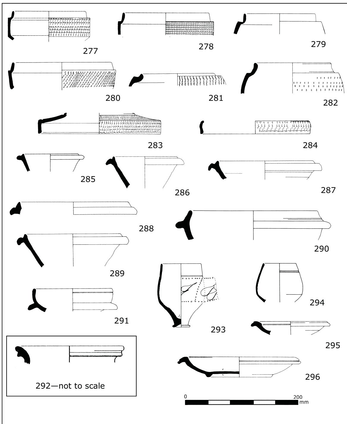
Fig. D9.51. Coarse pottery type series nos. 277-296. Scale 1:4 unless otherwise stated
