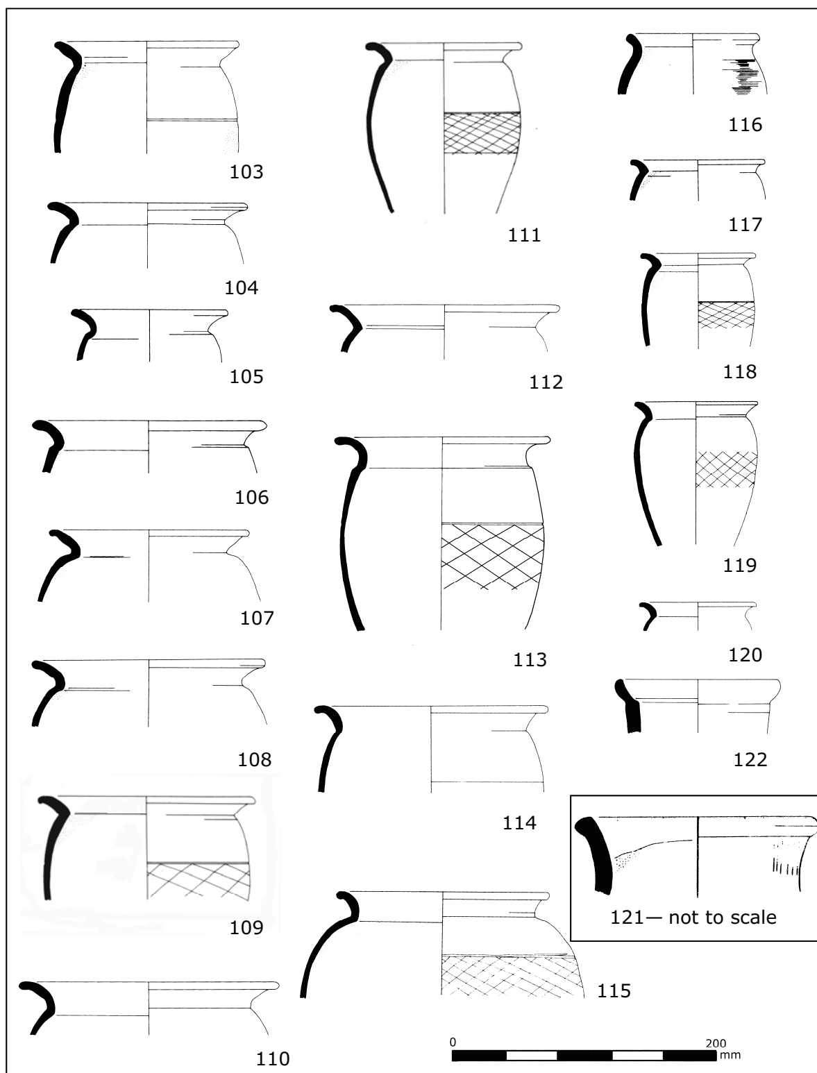
Fig. D9.42. Coarse pottery type series nos. 103—122. Scale 1:4 unless otherwise stated
