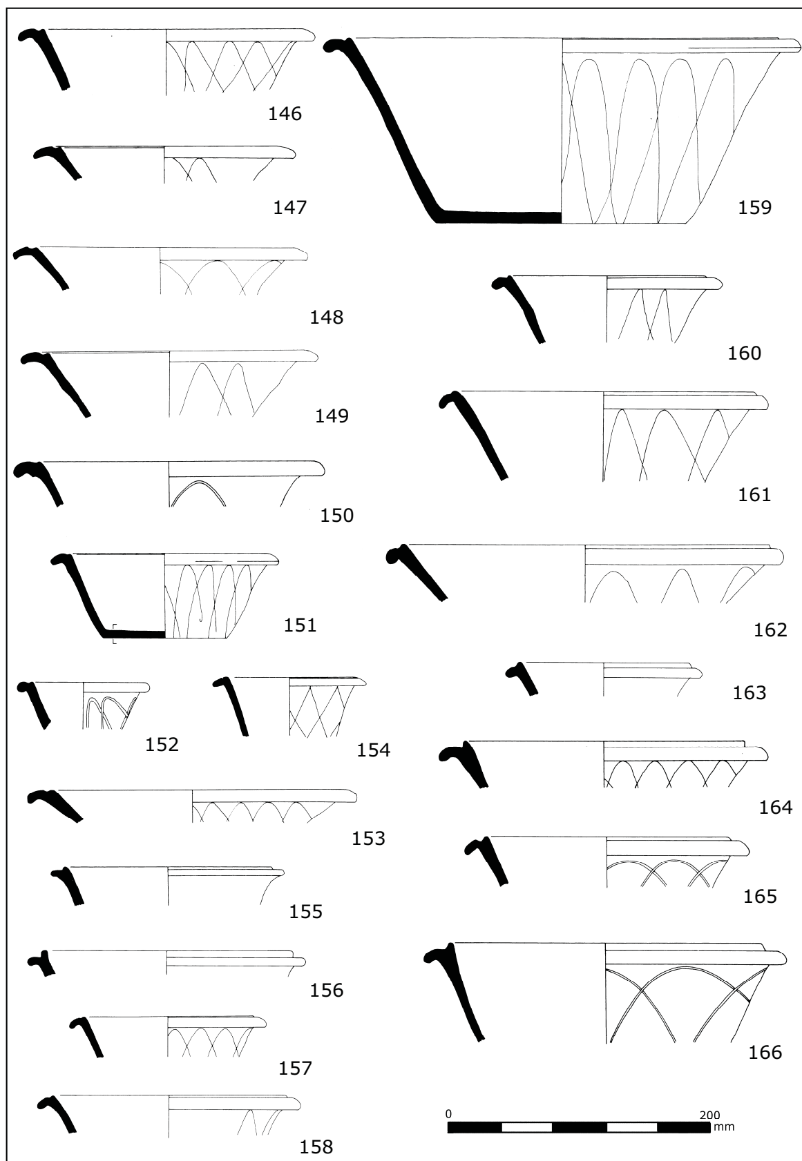
Fig. D9.44. Coarse pottery type series nos. 146—166. Scale 1:4
