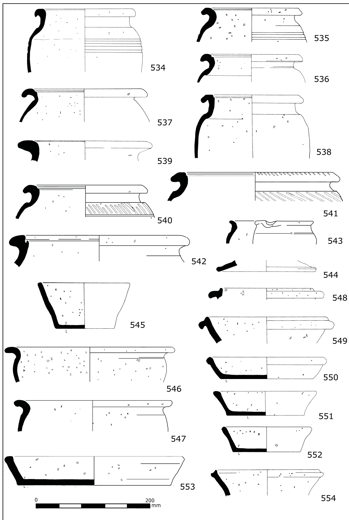
Fig. D9.62. Coarse pottery type series nos. 534-554. Scale 1:4
