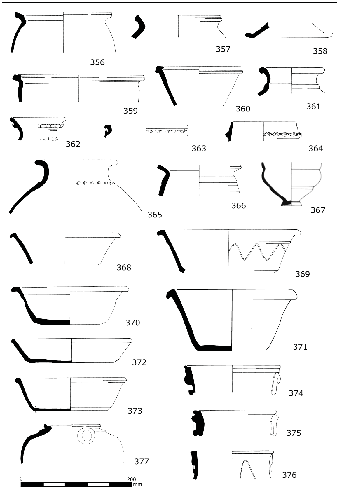
Fig. D9.54. Coarse pottery type series nos. 356-377. Scale 1:4.
