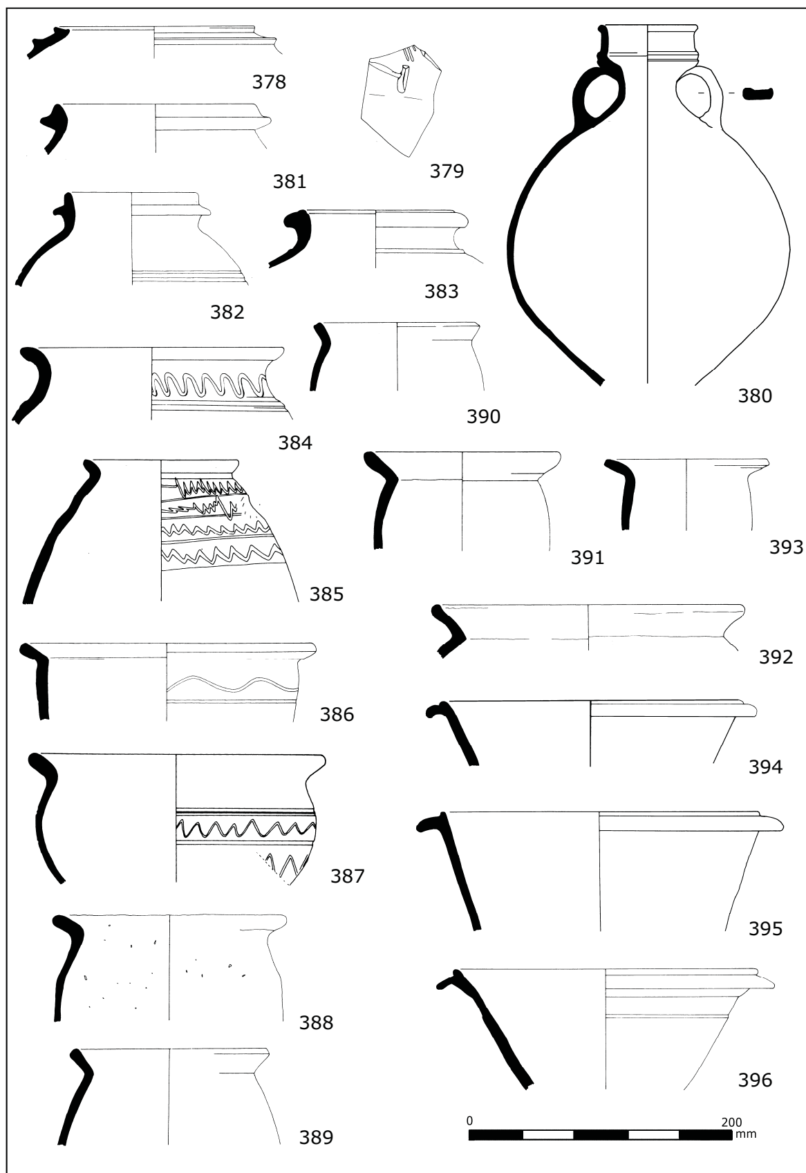
Fig. D9.55. Coarse pottery type series nos. 378-396. Scale 1:4.
