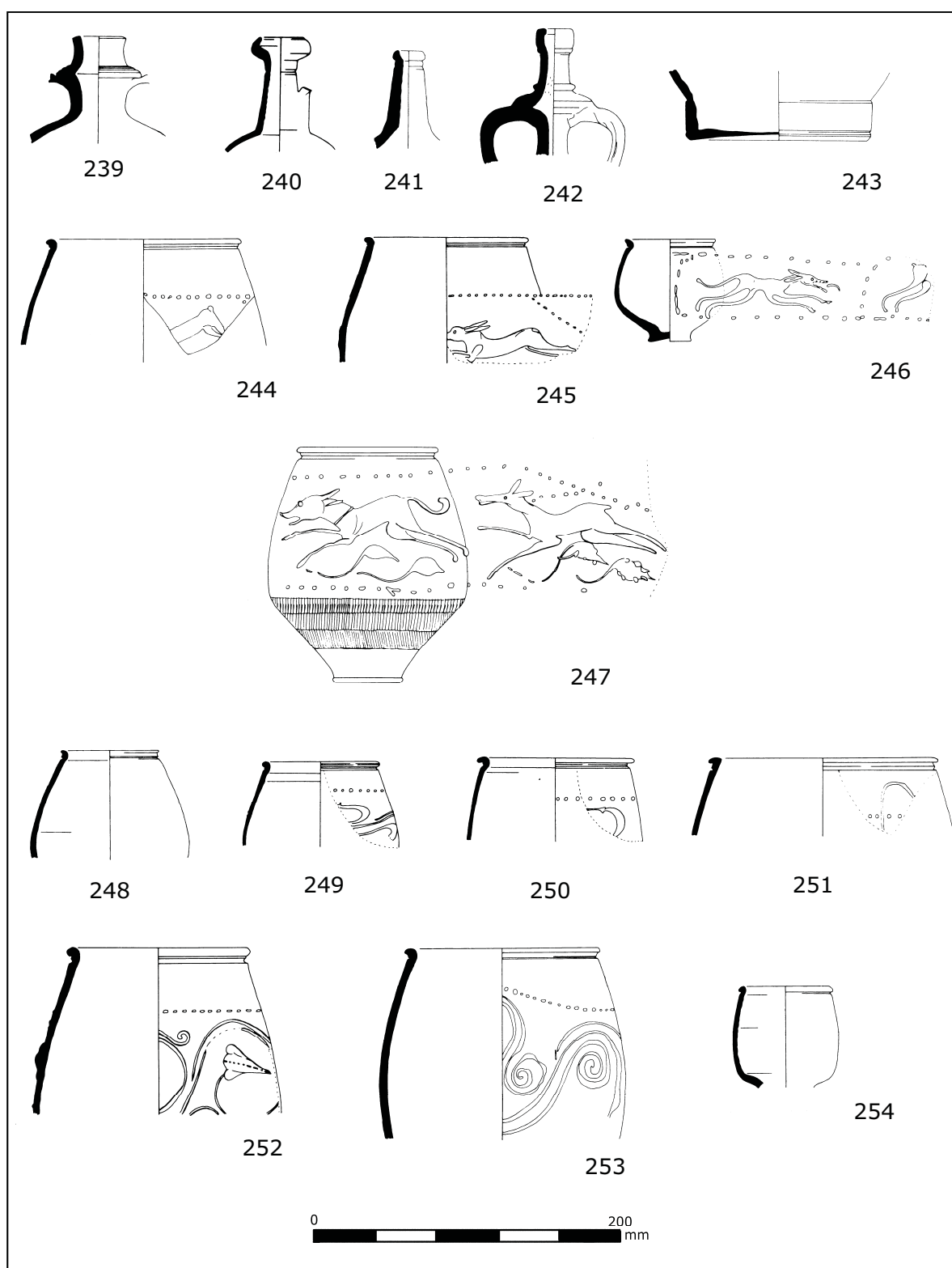
Fig. D9.49. Coarse pottery type series nos. 239-254. Scale 1:4.
