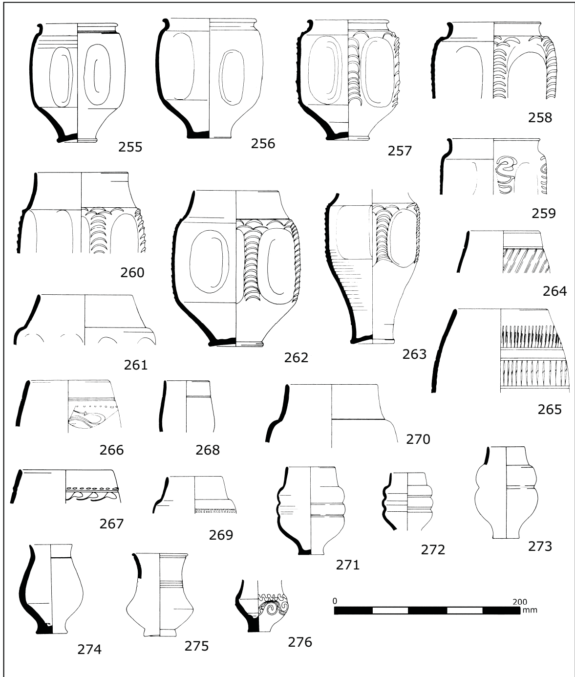
Fig. D9.50. Coarse pottery type series nos. 255-276. Scale 1:4.
