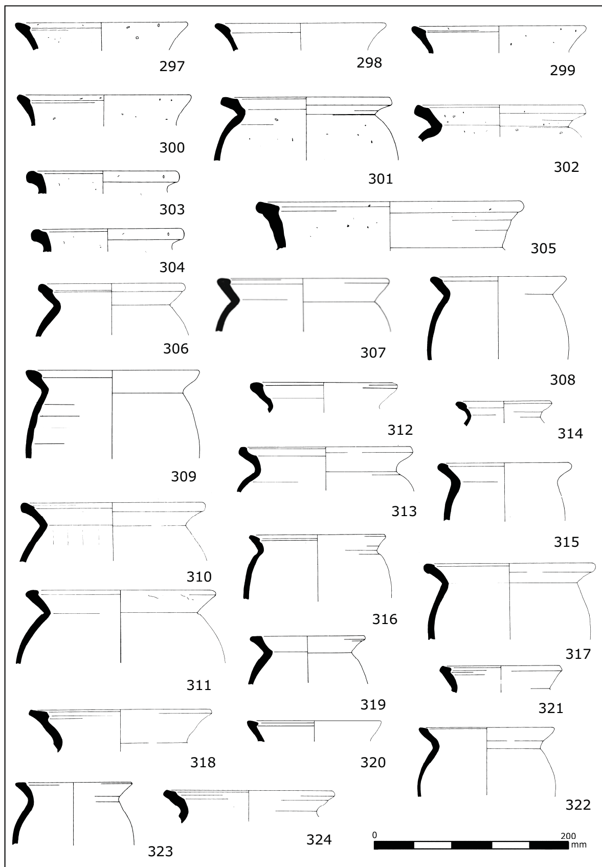
Fig. D9.52. Coarse pottery type series nos. 297-324. Scale 1:4.
