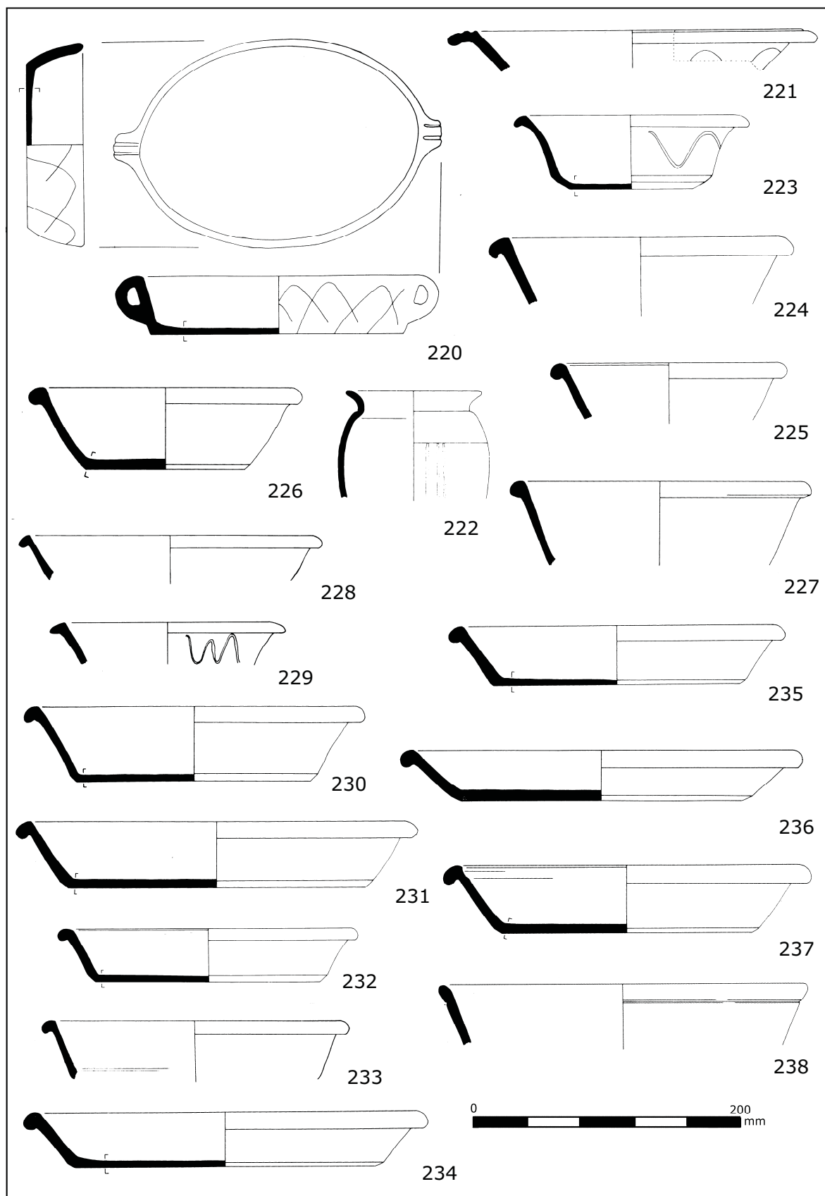
Fig. D9.48. Coarse pottery type series nos. 220-238. Scale 1:4
