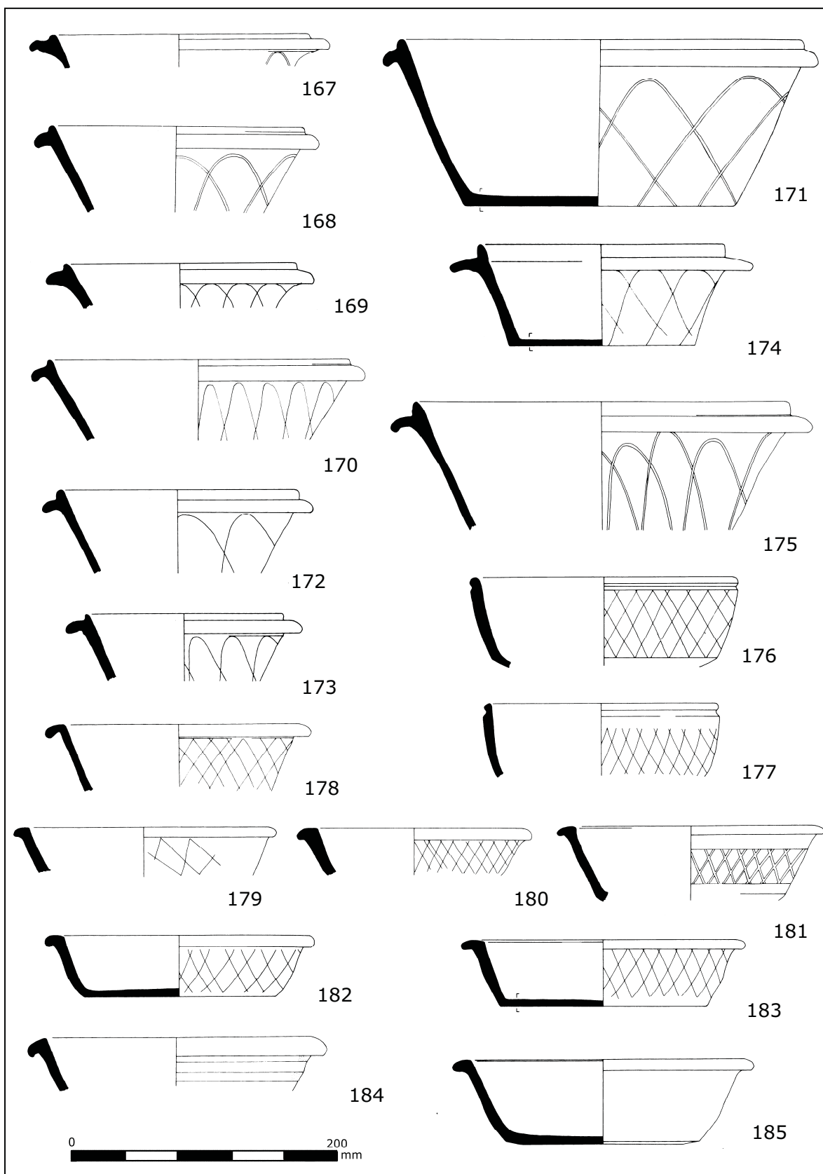
Fig. D9.45. Coarse pottery type series nos. 167-185. Scale 1:4.
