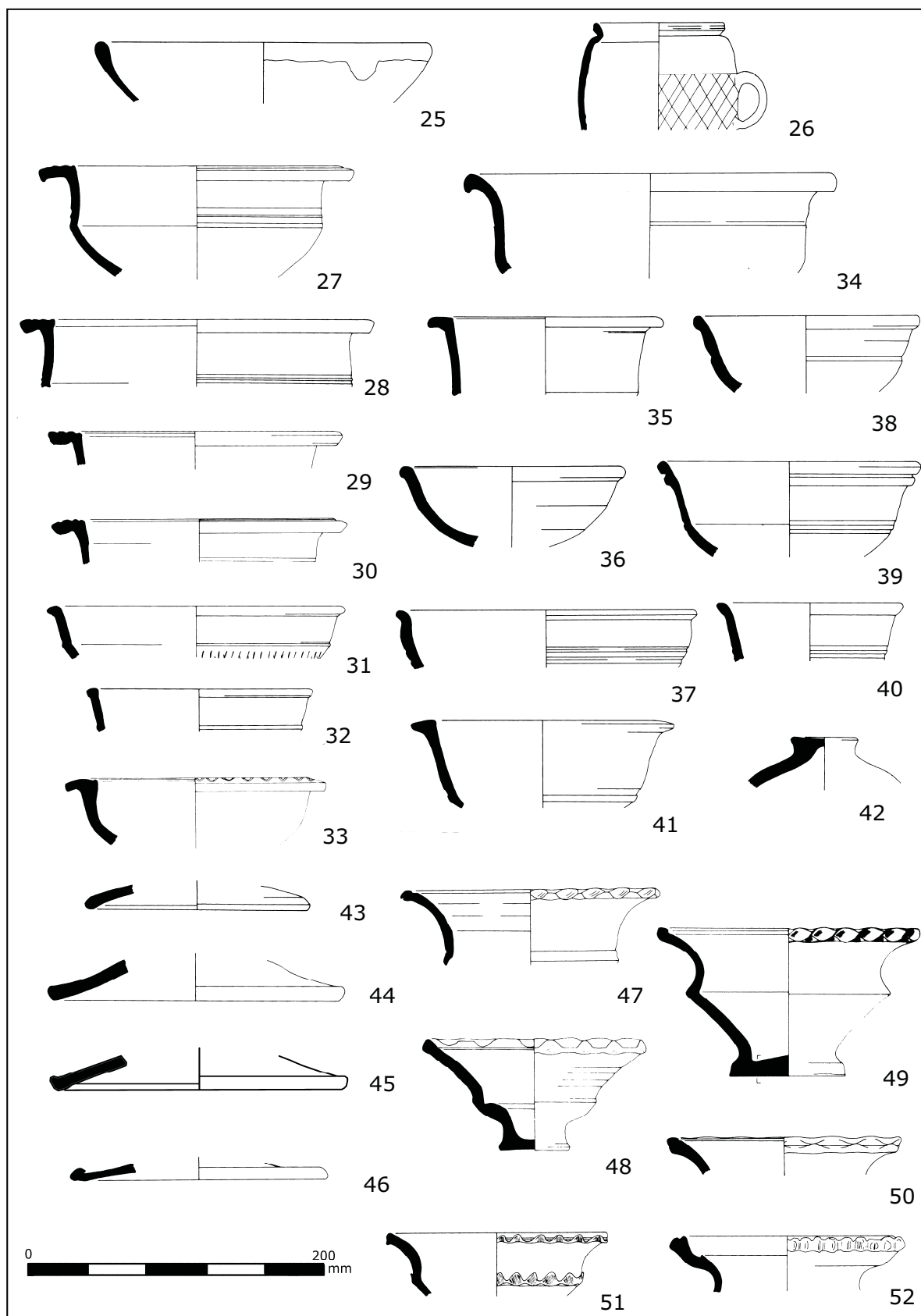
Fig. D9.39. Coarse pottery type series nos. 25-52. Scale 1:4
