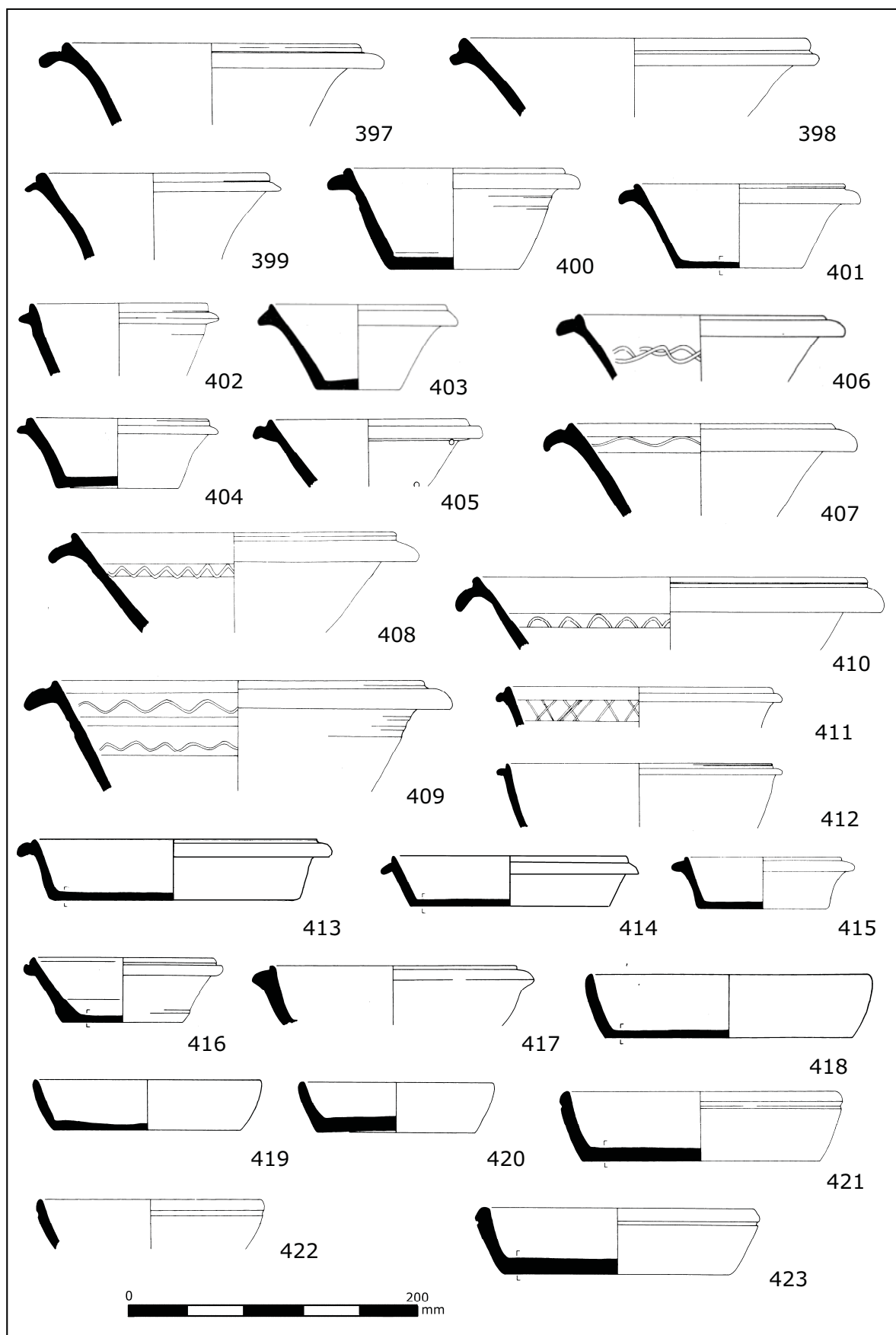
Fig. D9.56. Coarse pottery type series nos. 397-423. Scale 1:4.
