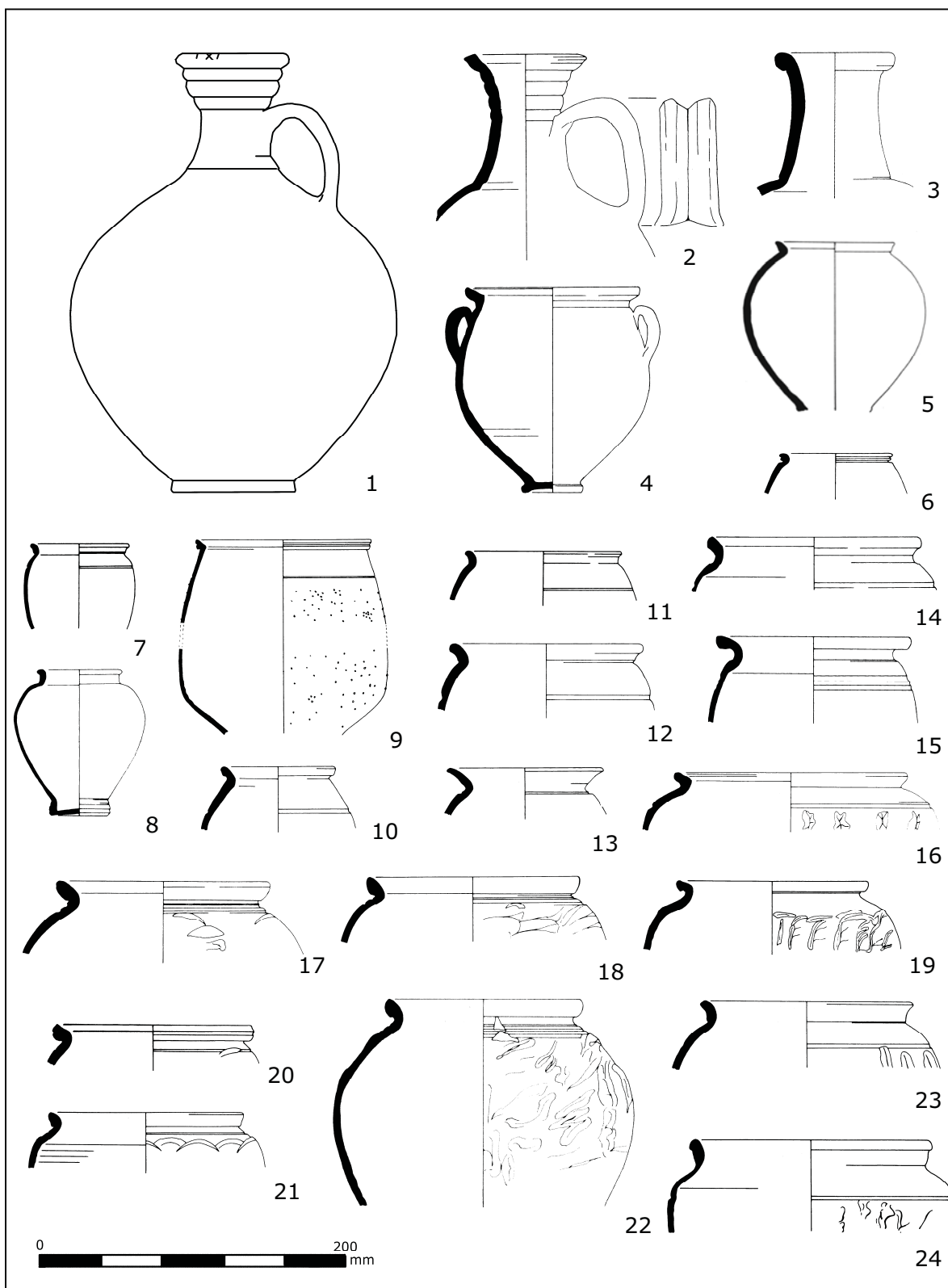
Fig. D9.38. Coarse pottery type series nos. 1-24. Scale 1:4
