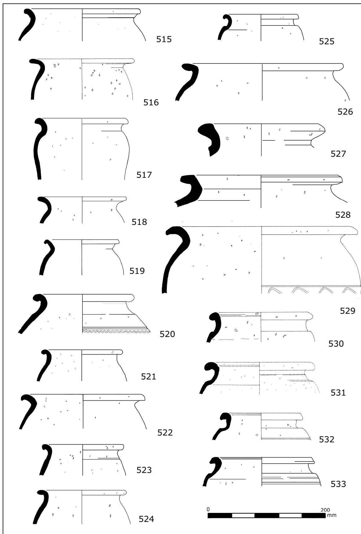
Fig. D9.61. Coarse pottery type series nos. 515-533. Scale 1:4.
