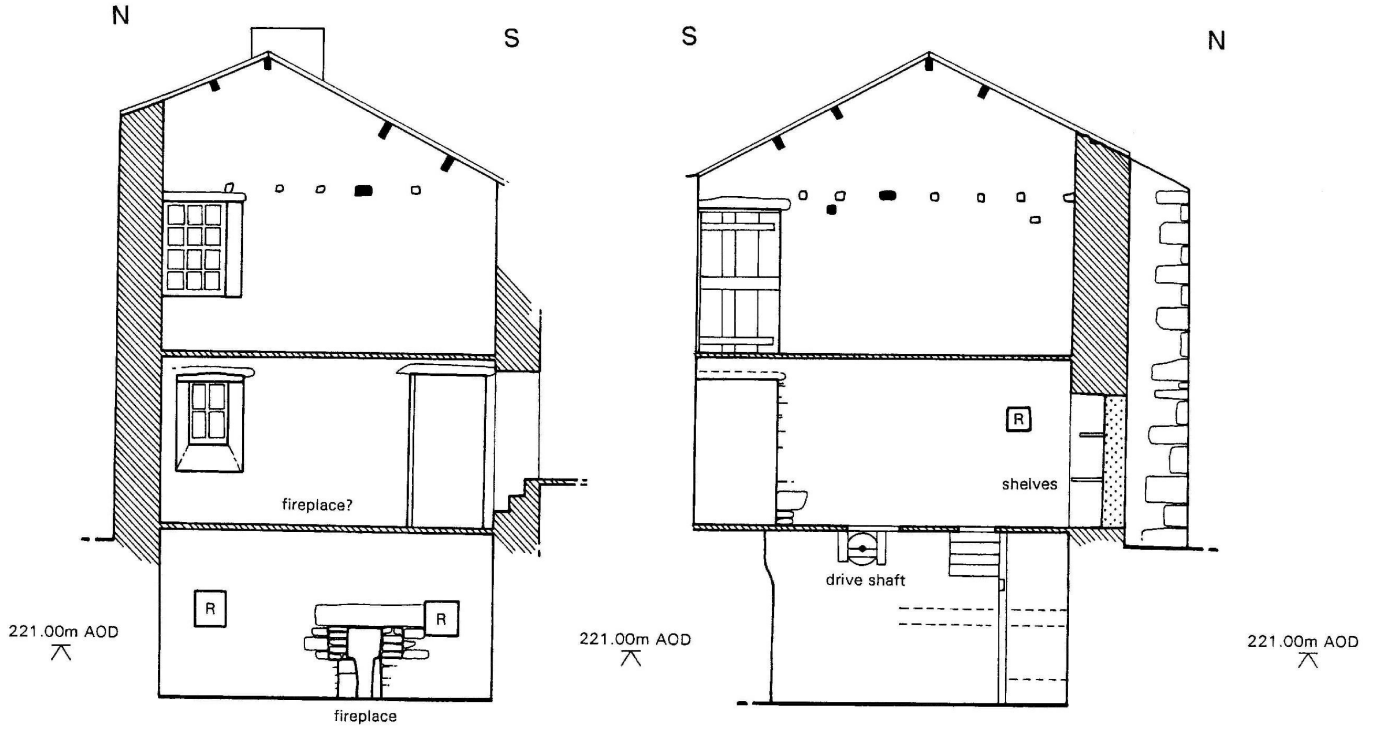
Elevation 15: east internal wall of 'domestic' end of mill
