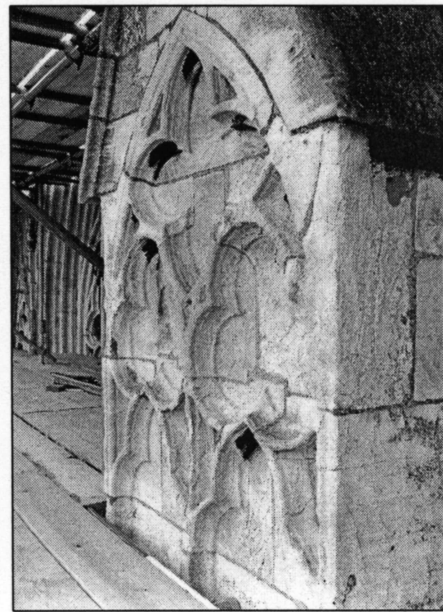
Photo 2/16: Top of blind arcading, south nave buttress, looking N.
