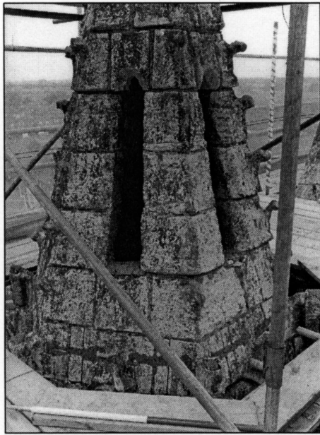
Photo 1/7: Spirelet of south nave turret, looking NW.
