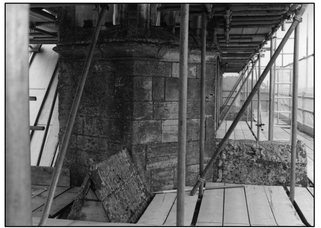
Photo 2/2: North nave turret base, looking S.
