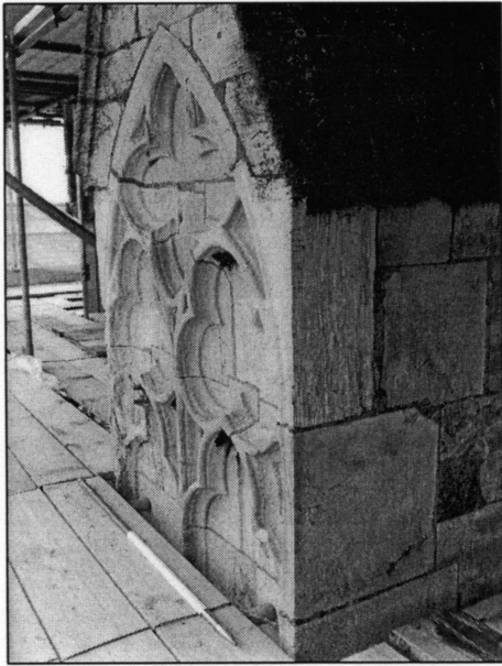
Photo 2/11: Top of Blind arcading, north nave buttress, looking N.
