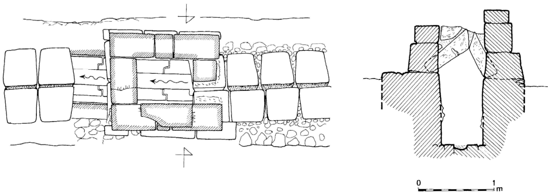
Fig. 6.25: Manhole in the Ramat Hanadiv aqueduct, Israel: view, plan and section [Hirschfeld 2002b, fig. 11a and b].
