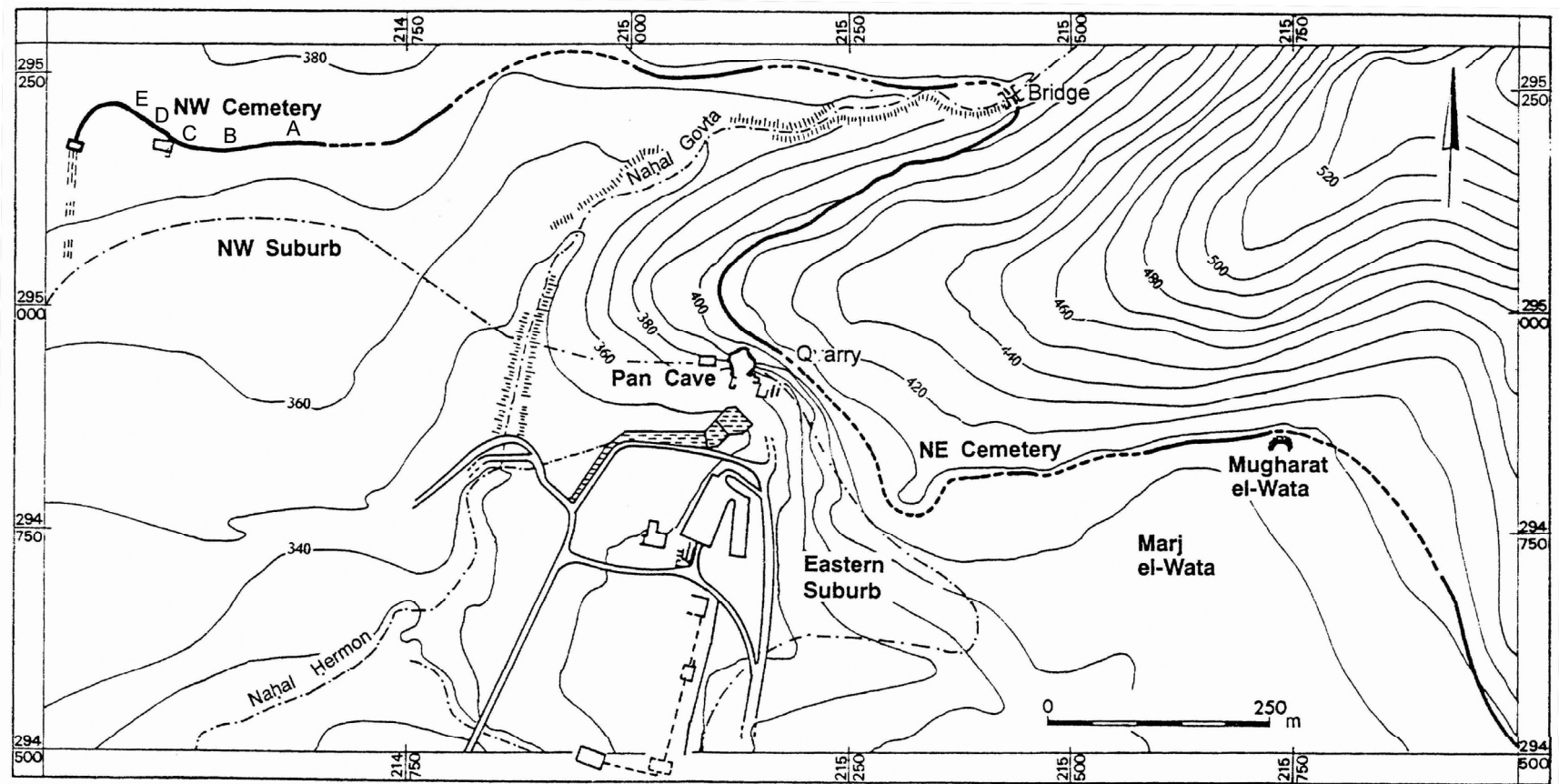
Fig. 7.6: Plan of the Baniyas aqueduct, Israel showing the probable locations (A-E), according to the description in the publication, of the distribution pools [after Hartal 2002, fig. 2].
