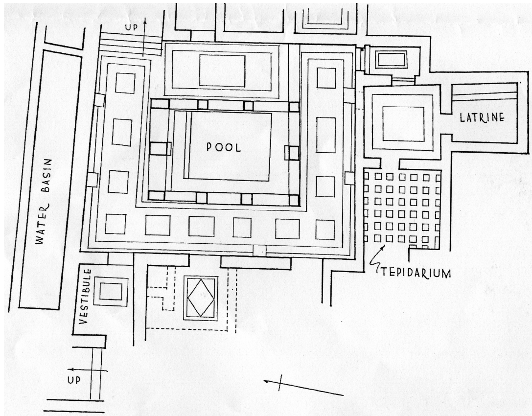
Fig. 8.24: Plan of the Jekmeje bathhouse, near Antioch. Scale 1:200 [Stillwell 1941, plan 6].
