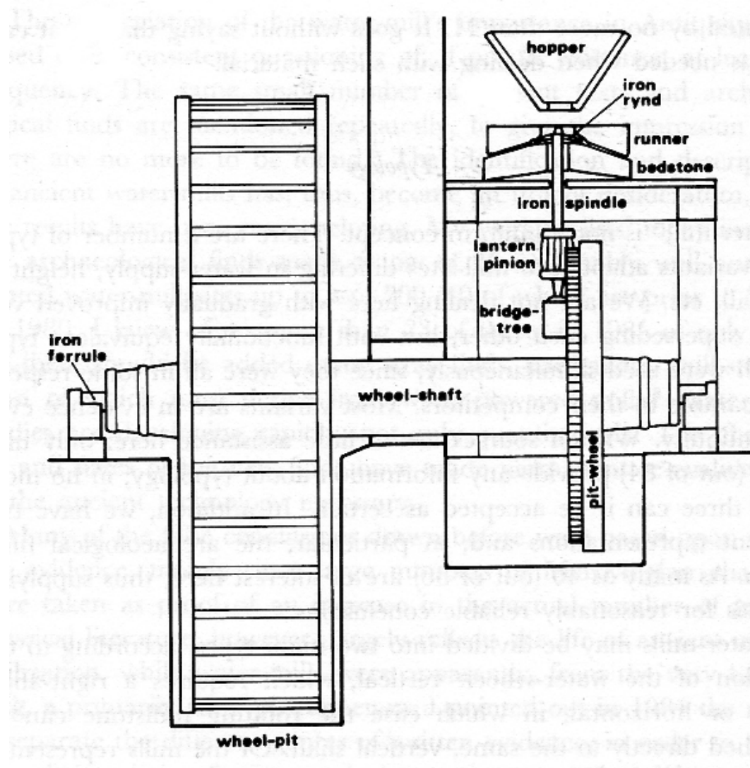
Fig. 10.1: Schematic drawing of vertical-wheeled, undershot mill [Wikander 2000b, fig. 1].
