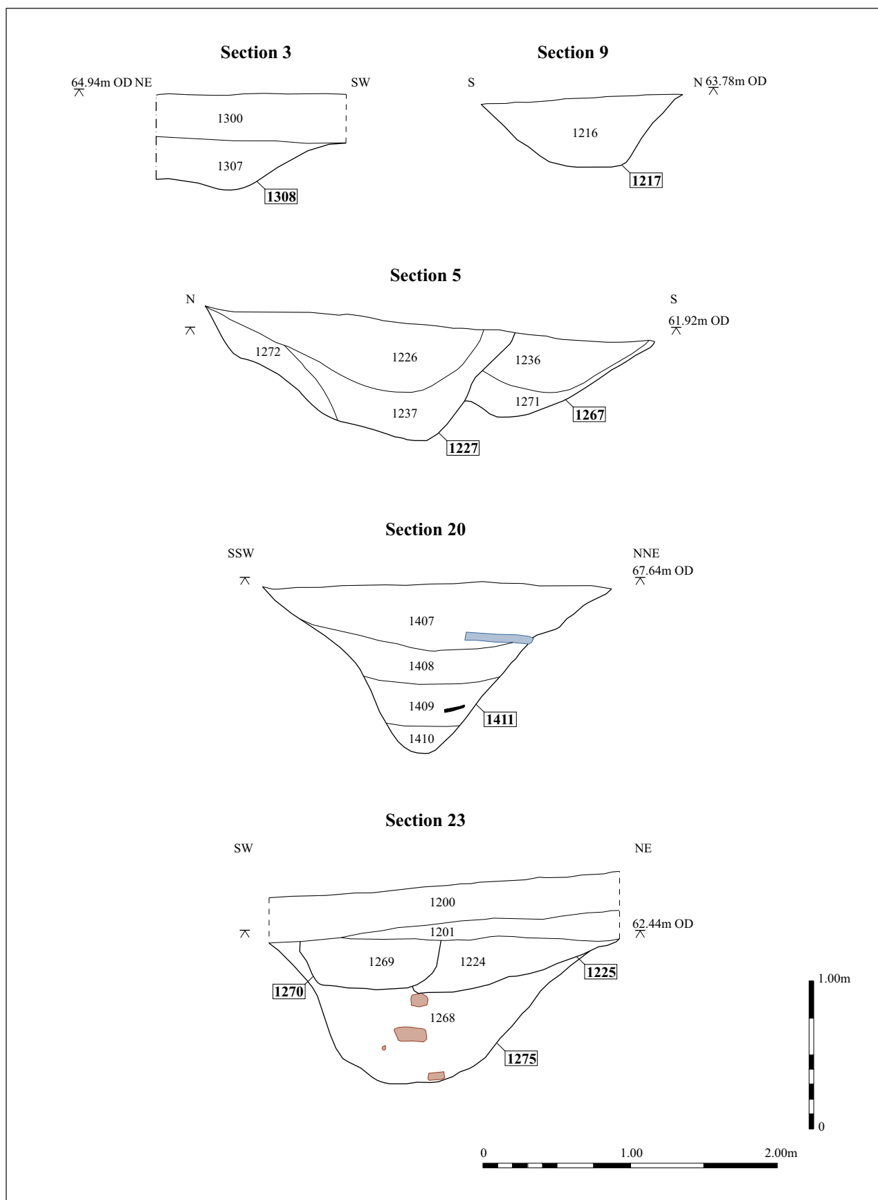
Figure 15: Sections from features in Trenches 12-14
