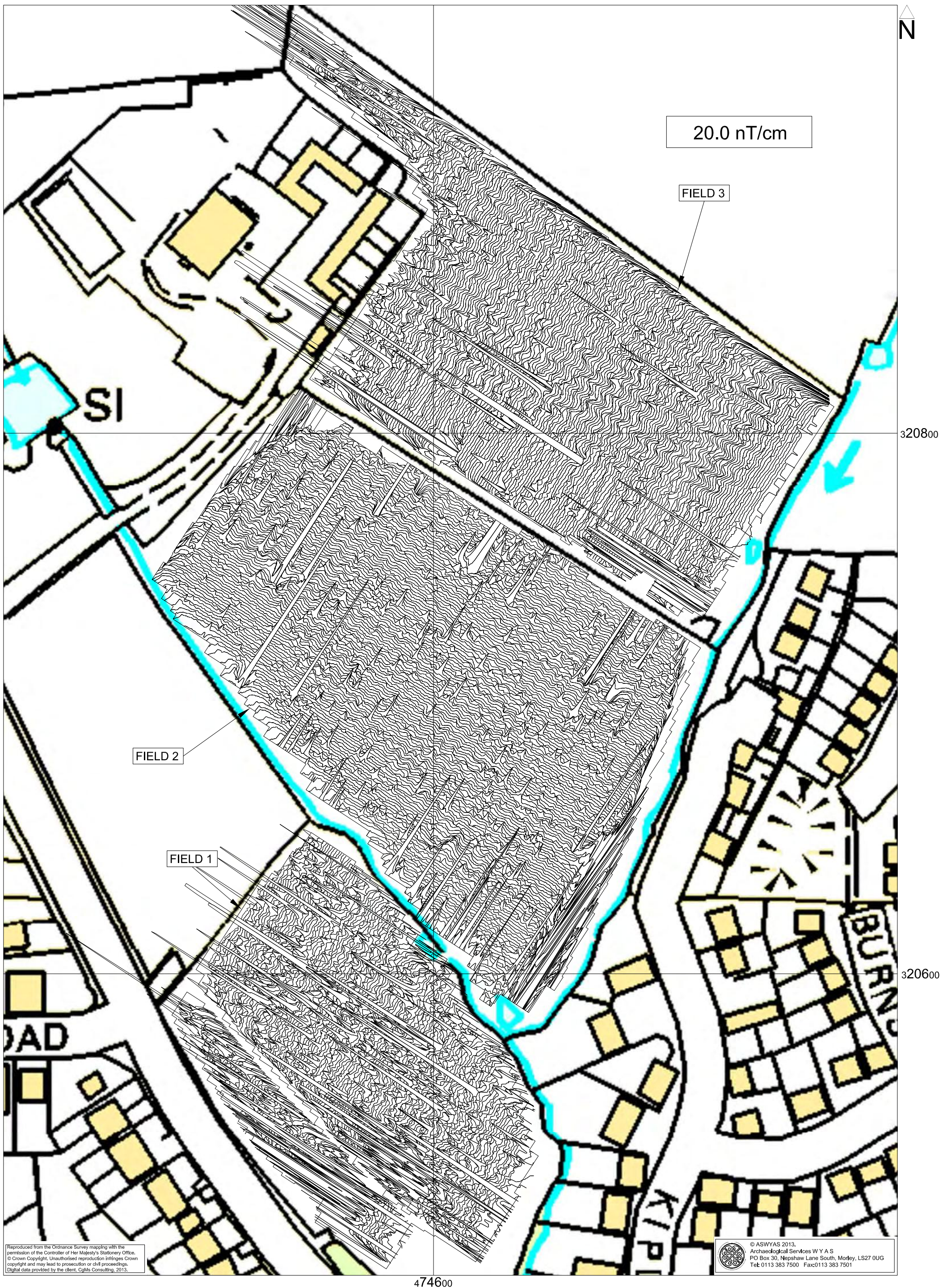
Fig. 4. XY trace plot of minimally processed magnetometer data (1:1250 @ A3)
