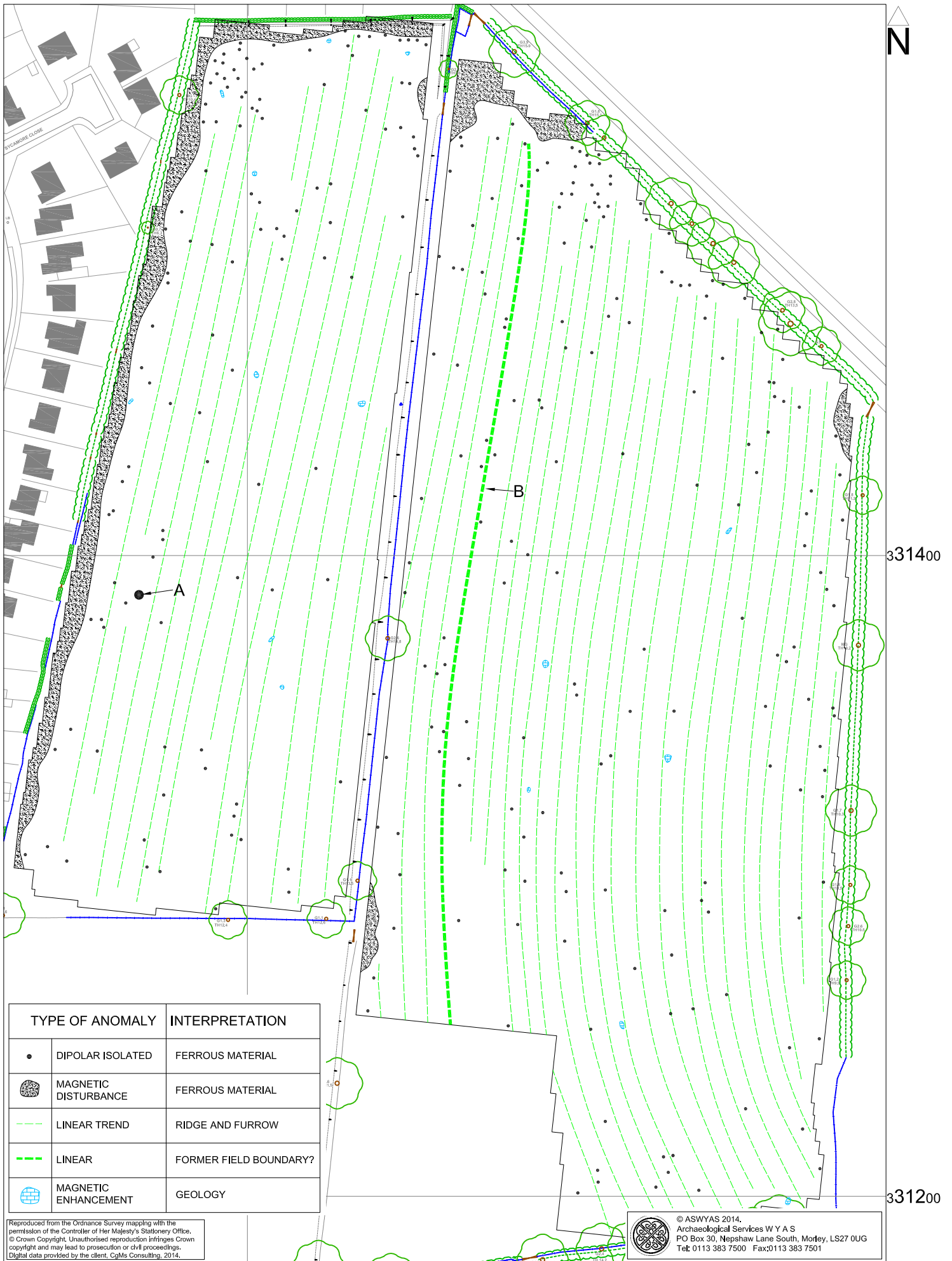
Fig. 5. Interpretation of magnetometer data (1:1500 @ A4)
