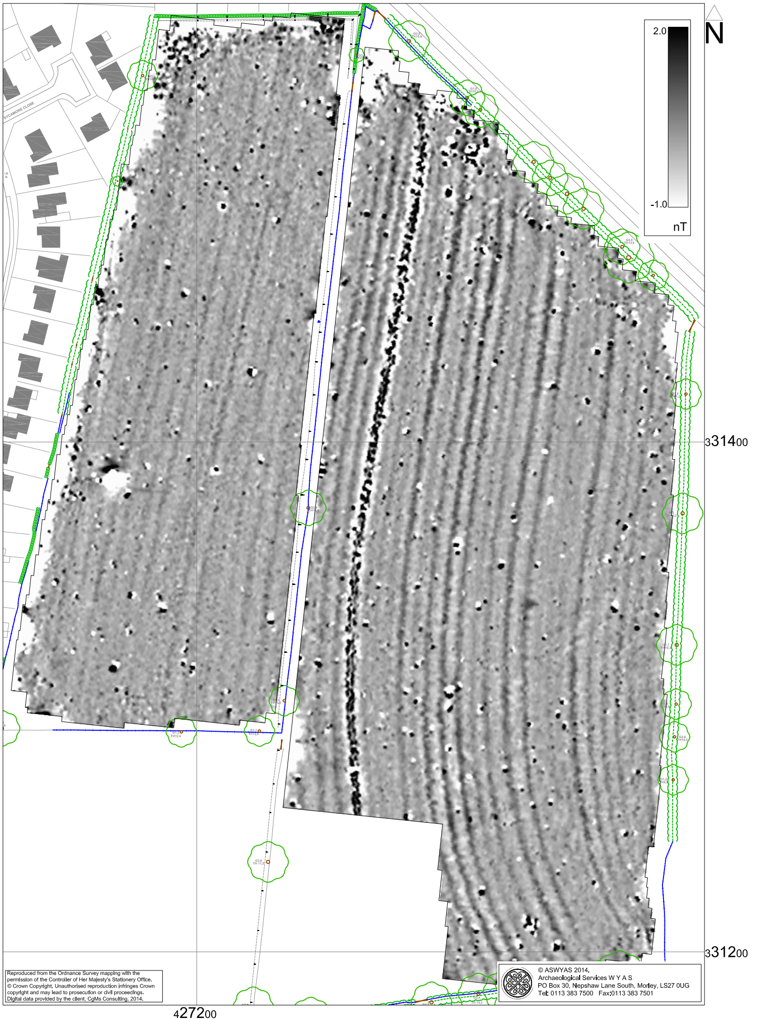
Fig. 3. Processed greyscale magnetometer data (1:1500 @ A4)
