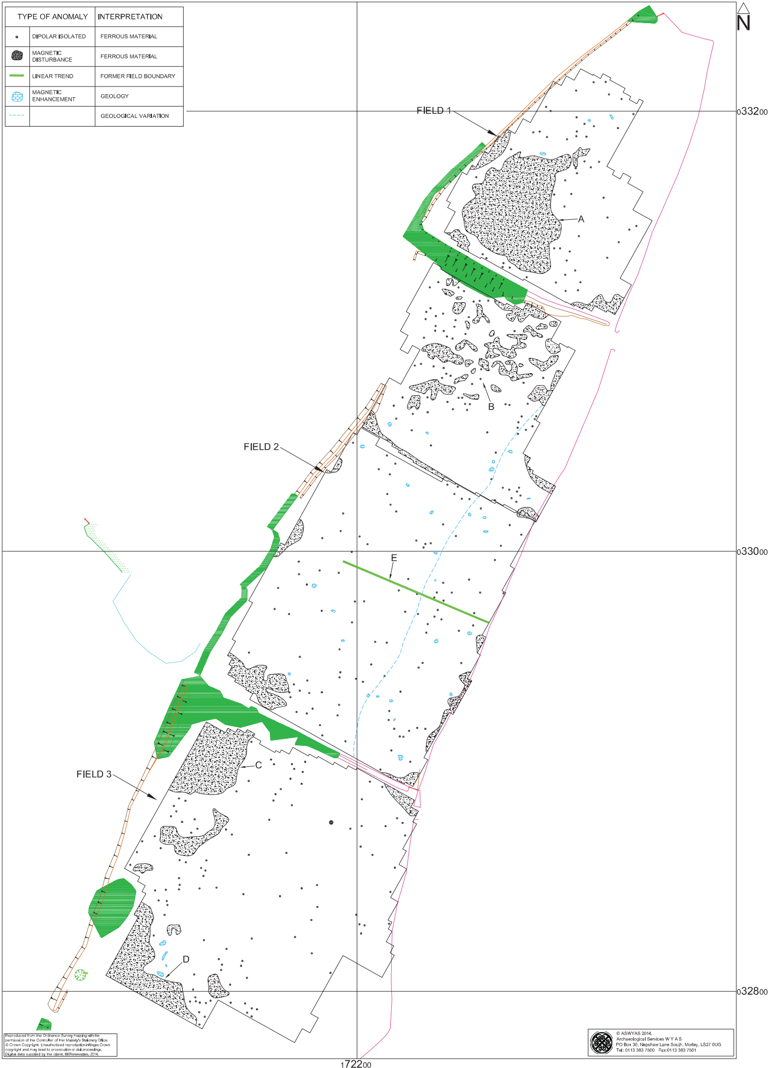
Fig. 5. Interpretation of magnetometer data (1:1250 @ A3)
