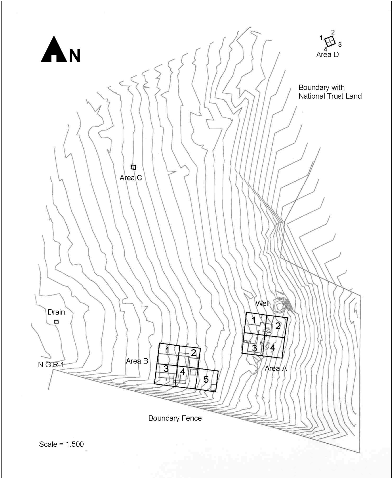
Figure D.2: Topographic survey, location of excavation trenches indicated.
