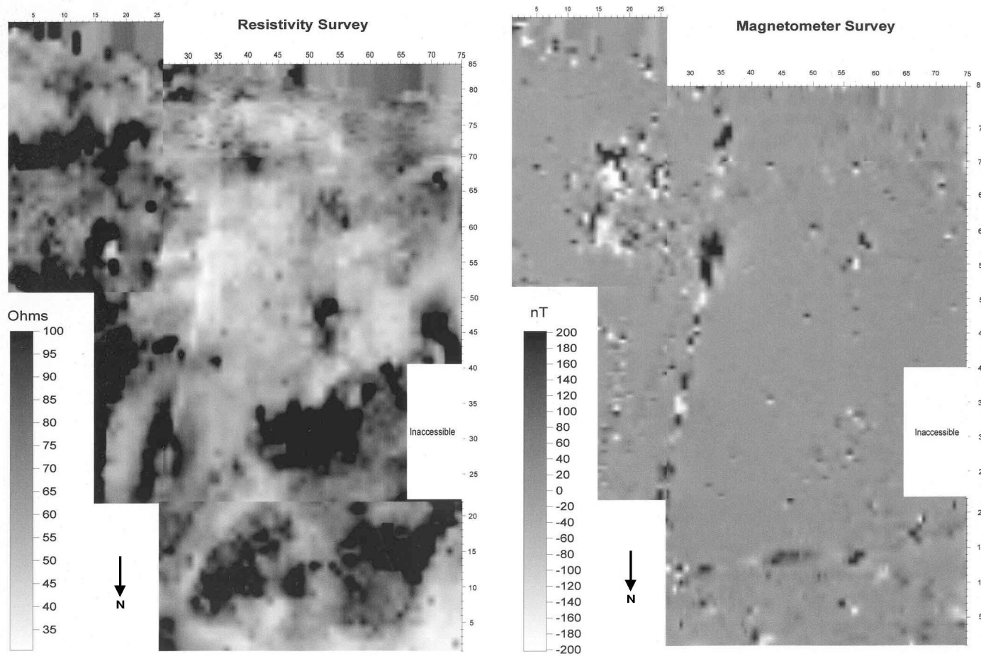
Figure D.3: Results of Electro-resistivity and Magnetometer Surveys.
