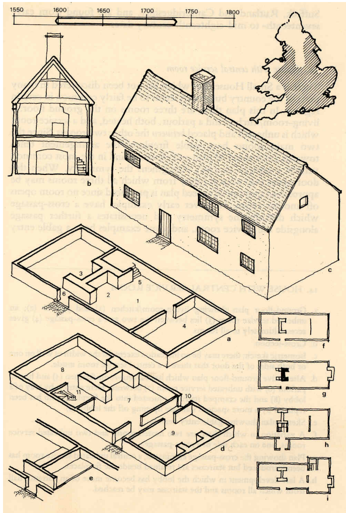
Figure E.12: Plan of typical rural cottage, c.1600 – 1740 (Brunskill 1982).
