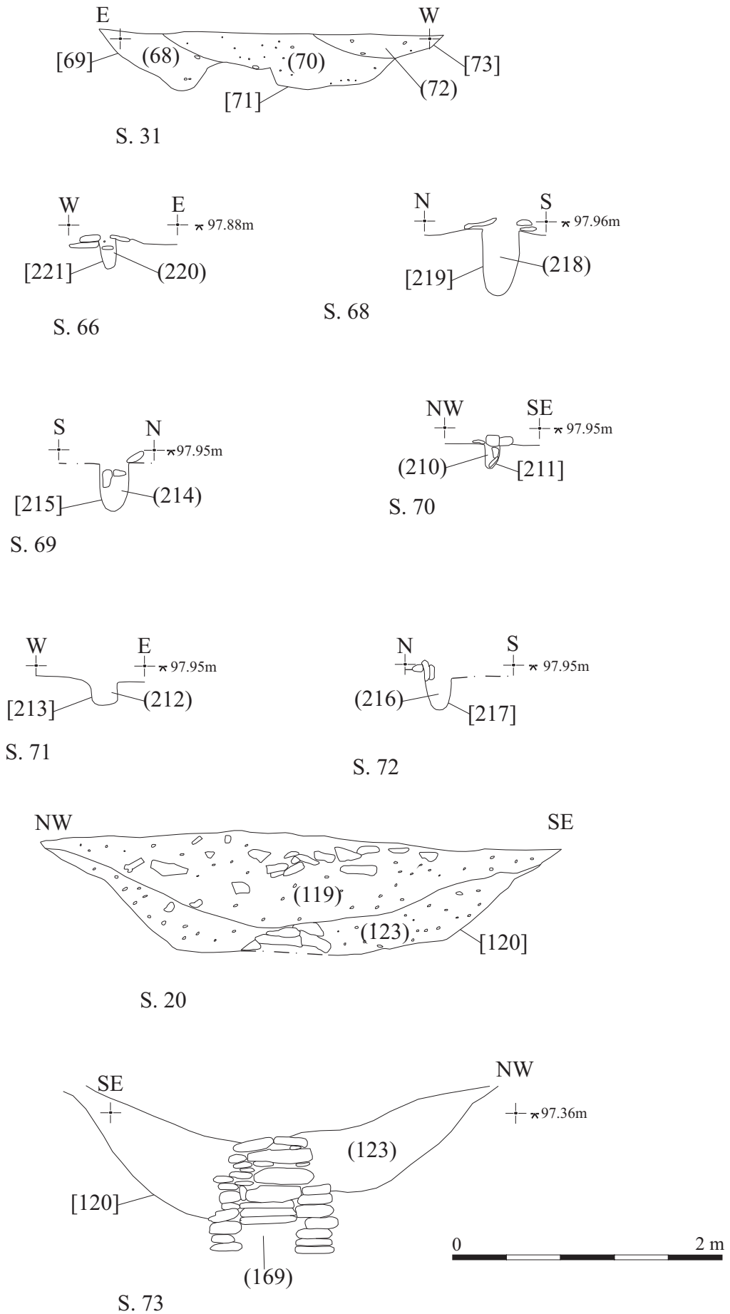
Figure 11. Phase 3 sections
